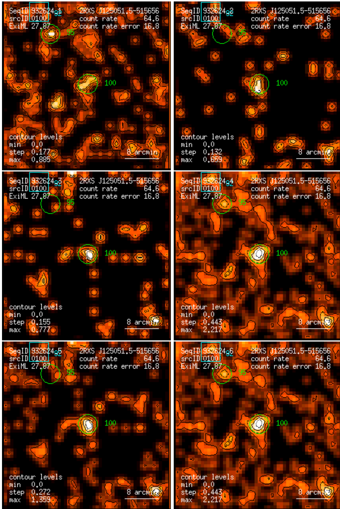
Figure 100: RASS 932624: detection 0100: band rate images, Gaussian filter: (1) PSPC channels 11 – 41, (2) 52 – 90, (3) 91 – 201, (4) 11 – 235, (5) 52 – 201, (6) 11 – 201. Broad band rates in counts/ks. Band rate contour levels in counts/ks/arcmin 2 .
