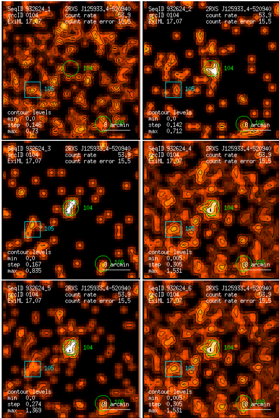
Figure 104: RASS 932624: detection 0104: band rate images, Gaussian filter: (1) PSPC channels 11 – 41, (2) 52 – 90, (3) 91 – 201, (4) 11 – 235, (5) 52 – 201, (6) 11 – 201. Broad band rates in counts/ks. Band rate contour levels in counts/ks/arcmin 2 .
