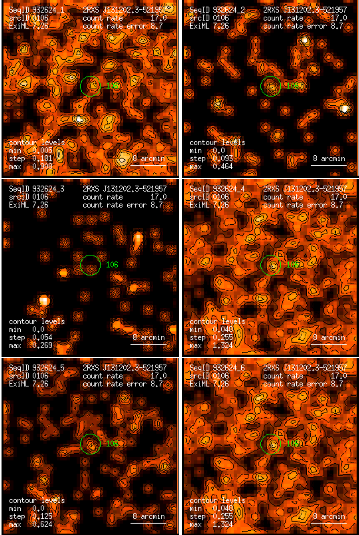
Figure 106: RASS 932624: detection 0106: band rate images, Gaussian filter: (1) PSPC channels 11 – 41, (2) 52 – 90, (3) 91 – 201, (4) 11 – 235, (5) 52 – 201, (6) 11 – 201. Broad band rates in counts/ks. Band rate contour levels in counts/ks/arcmin 2 .
