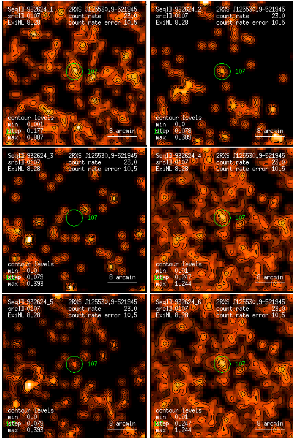
Figure 107: RASS 932624: detection 0107: band rate images, Gaussian filter: (1) PSPC channels 11 – 41, (2) 52 – 90, (3) 91 – 201, (4) 11 – 235, (5) 52 – 201, (6) 11 – 201. Broad band rates in counts/ks. Band rate contour levels in counts/ks/arcmin 2 .
