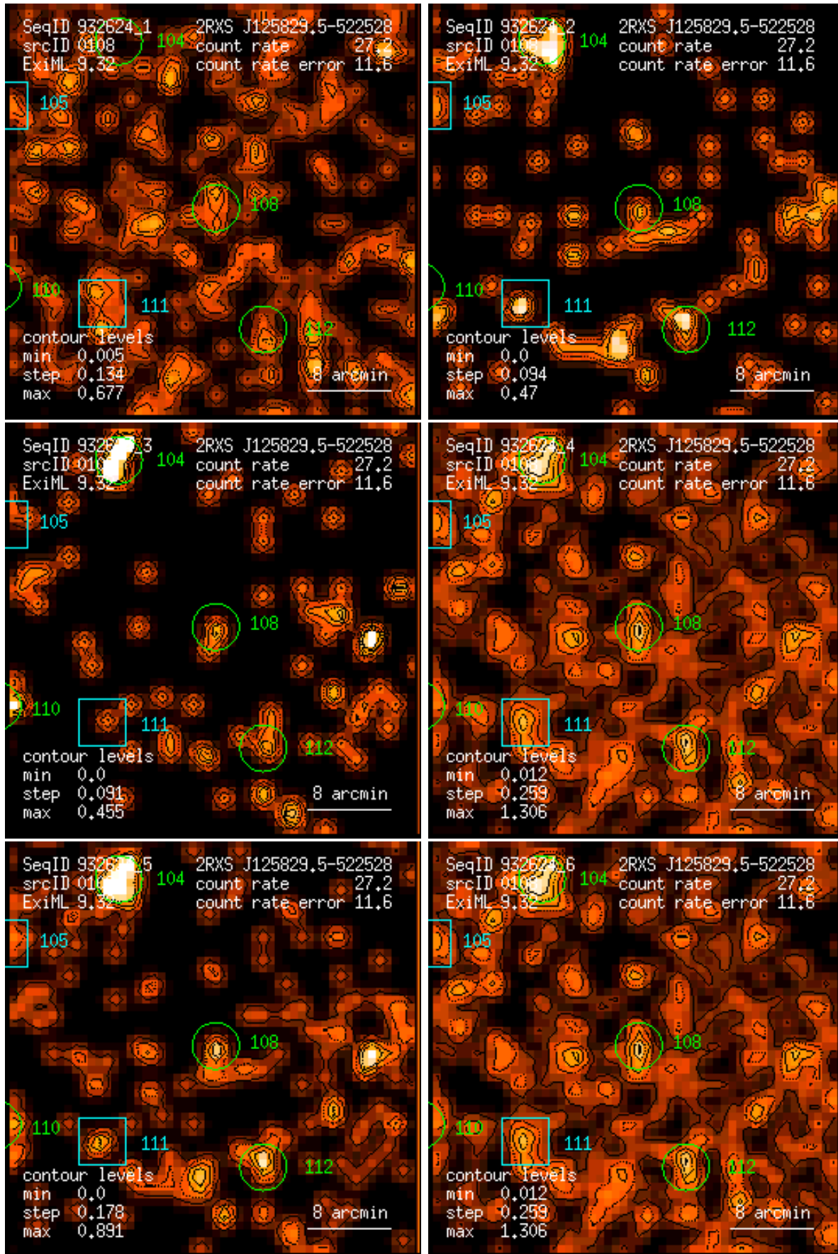
Figure 108: RASS 932624: detection 0108: band rate images, Gaussian filter: (1) PSPC channels 11 – 41, (2) 52 – 90, (3) 91 – 201, (4) 11 – 235, (5) 52 – 201, (6) 11 – 201. Broad band rates in counts/ks. Band rate contour levels in counts/ks/arcmin 2 .
