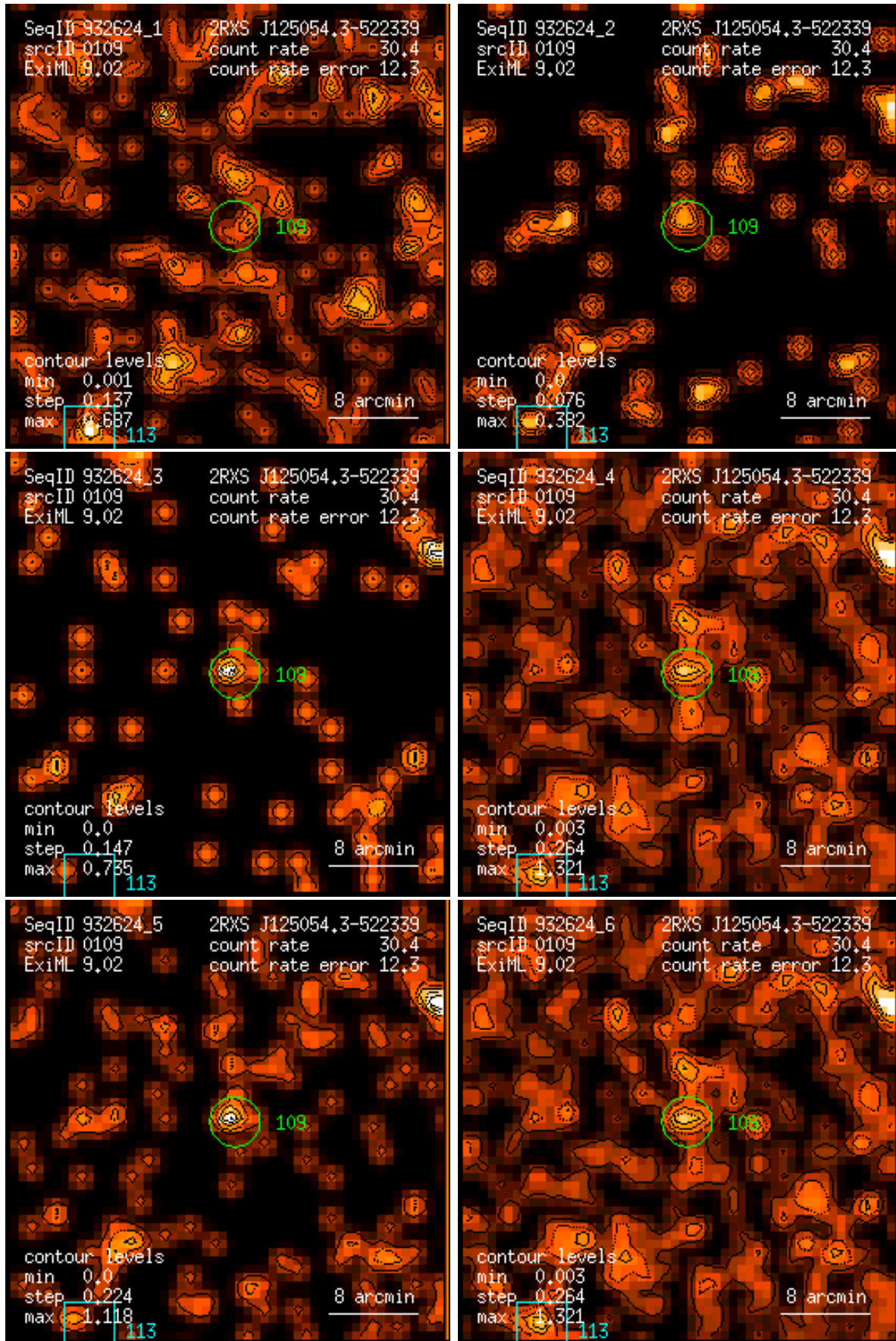
Figure 109: RASS 932624: detection 0109: band rate images, Gaussian filter: (1) PSPC channels 11 – 41, (2) 52 – 90, (3) 91 – 201, (4) 11 – 235, (5) 52 – 201, (6) 11 – 201. Broad band rates in counts/ks. Band rate contour levels in counts/ks/arcmin 2 .
