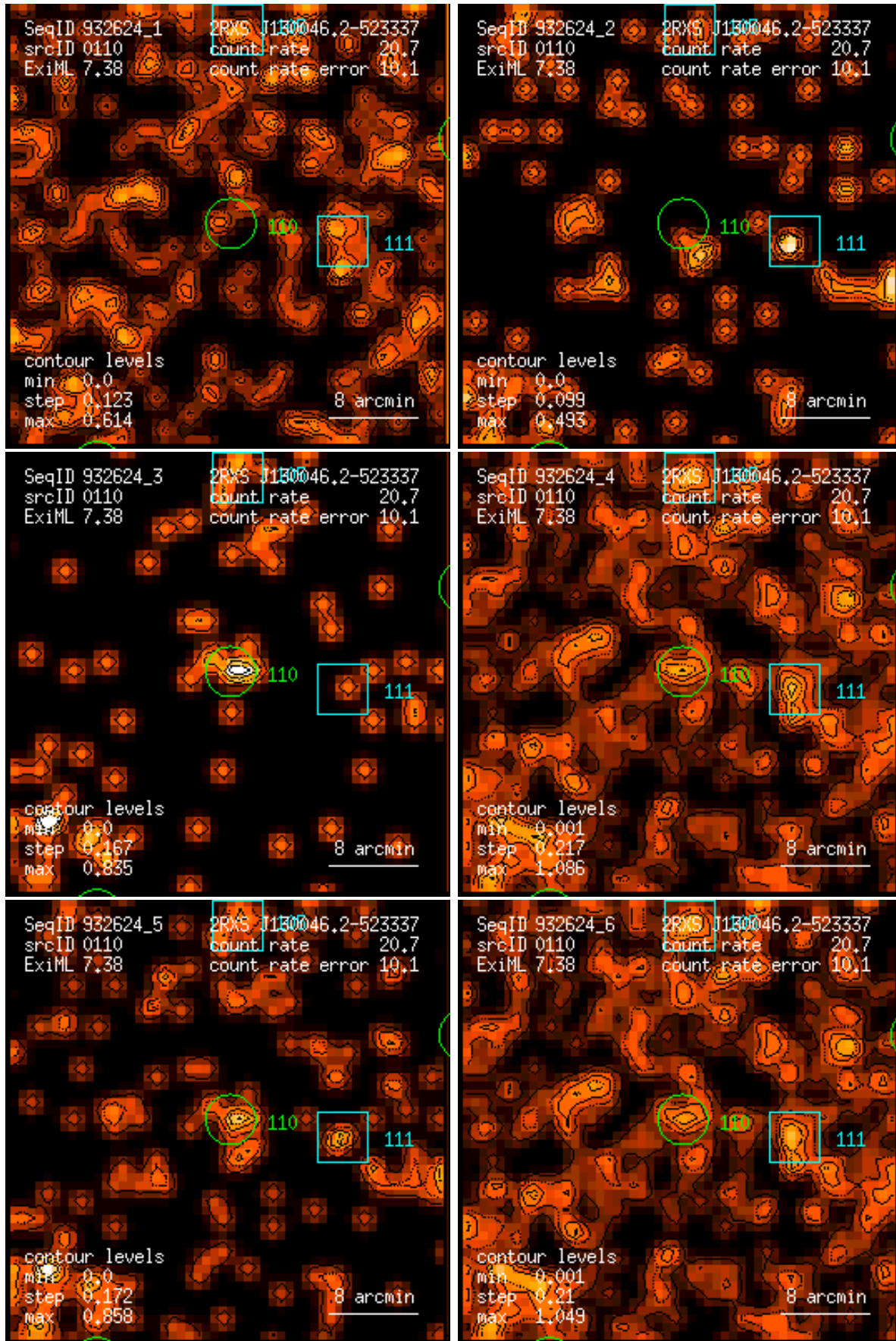
Figure 110: RASS 932624: detection 0110: band rate images, Gaussian filter: (1) PSPC channels 11 – 41, (2) 52 – 90, (3) 91 – 201, (4) 11 – 235, (5) 52 – 201, (6) 11 – 201. Broad band rates in counts/ks. Band rate contour levels in counts/ks/arcmin 2 .
