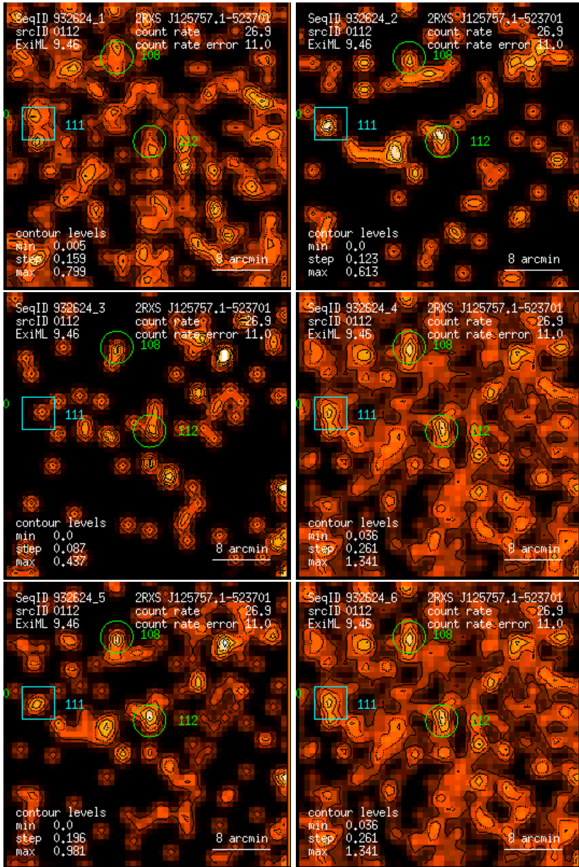
Figure 112: RASS 932624: detection 0112: band rate images, Gaussian filter: (1) PSPC channels 11 – 41, (2) 52 – 90, (3) 91 – 201, (4) 11 – 235, (5) 52 – 201, (6) 11 – 201. Broad band rates in counts/ks. Band rate contour levels in counts/ks/arcmin 2 .
