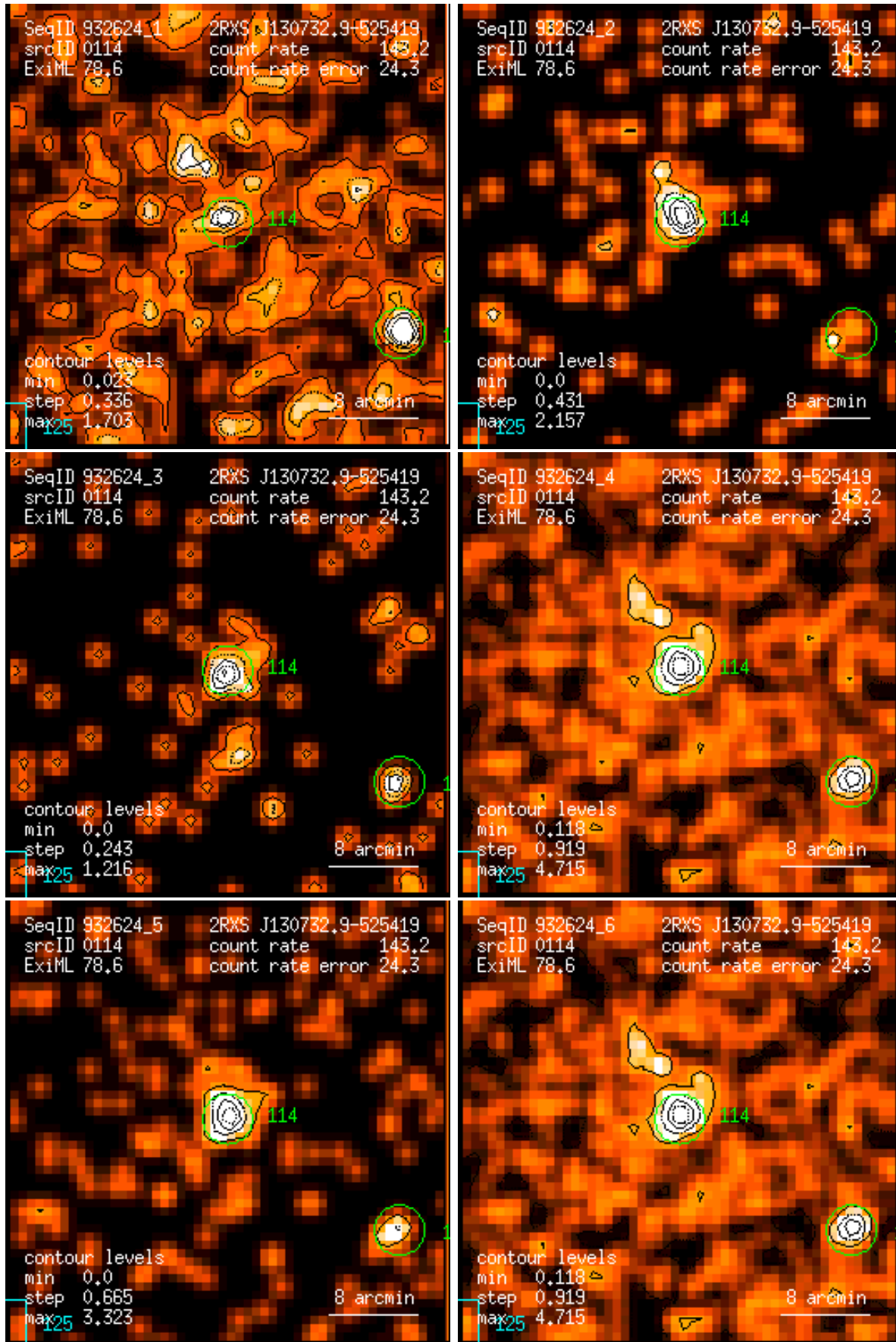
Figure 114: RASS 932624: detection 0114: band rate images, Gaussian filter: (1) PSPC channels 11 – 41, (2) 52 – 90, (3) 91 – 201, (4) 11 – 235, (5) 52 – 201, (6) 11 – 201. Broad band rates in counts/ks. Band rate contour levels in counts/ks/arcmin 2 .
