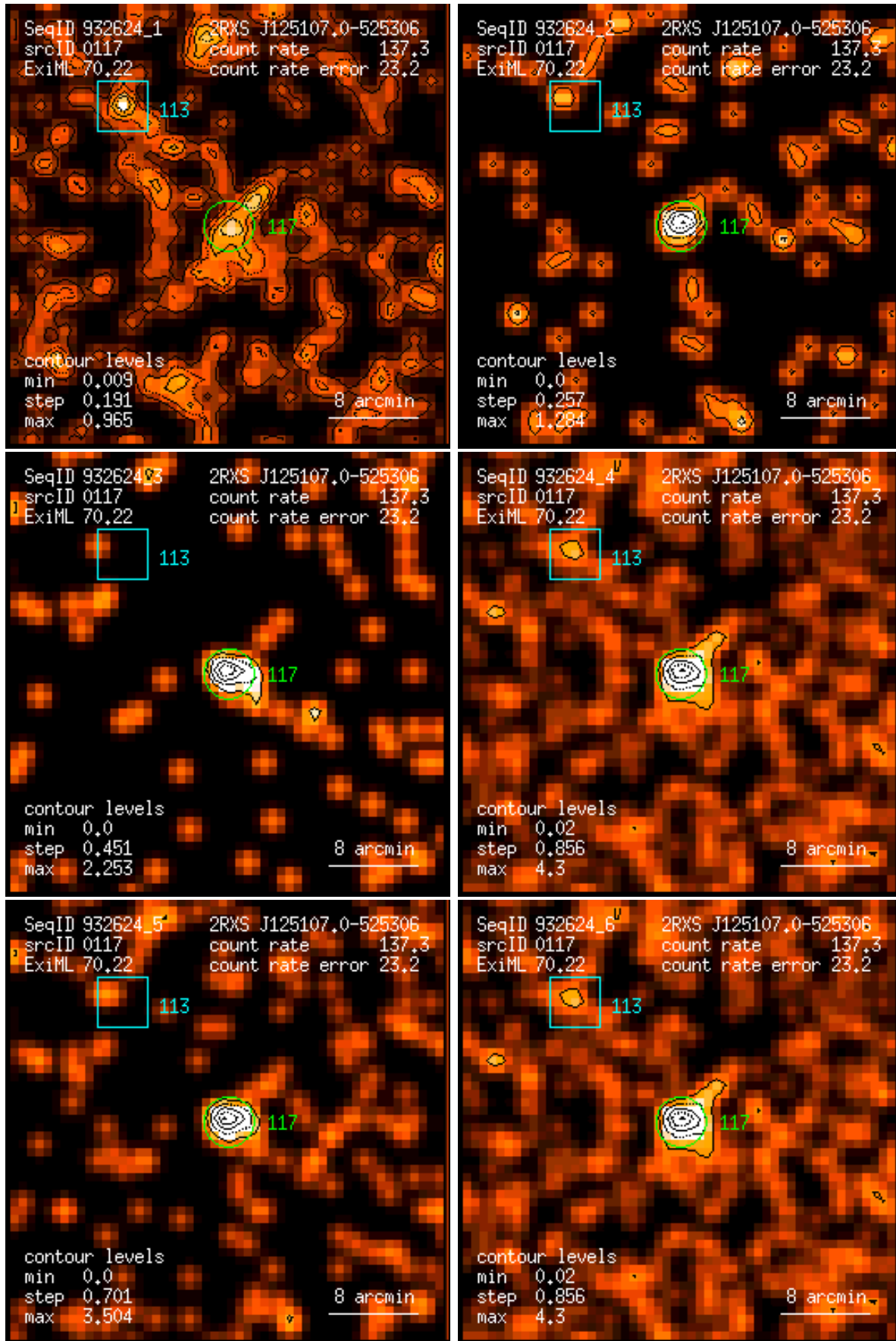
Figure 117: RASS 932624: detection 0117: band rate images, Gaussian filter: (1) PSPC channels 11 – 41, (2) 52 – 90, (3) 91 – 201, (4) 11 – 235, (5) 52 – 201, (6) 11 – 201. Broad band rates in counts/ks. Band rate contour levels in counts/ks/arcmin 2 .
