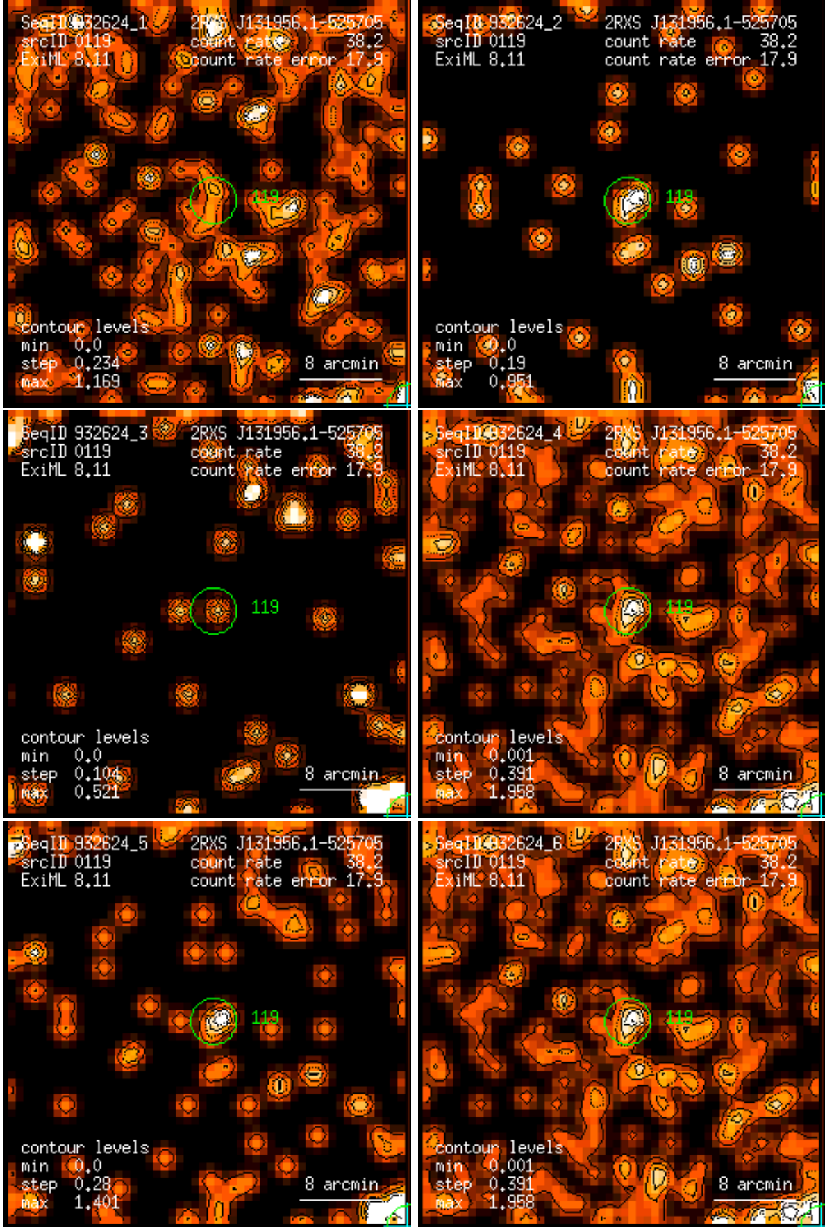
Figure 119: RASS 932624: detection 0119: band rate images, Gaussian filter: (1) PSPC channels 11 – 41, (2) 52 – 90, (3) 91 – 201, (4) 11 – 235, (5) 52 – 201, (6) 11 – 201. Broad band rates in counts/ks. Band rate contour levels in counts/ks/arcmin 2 .
