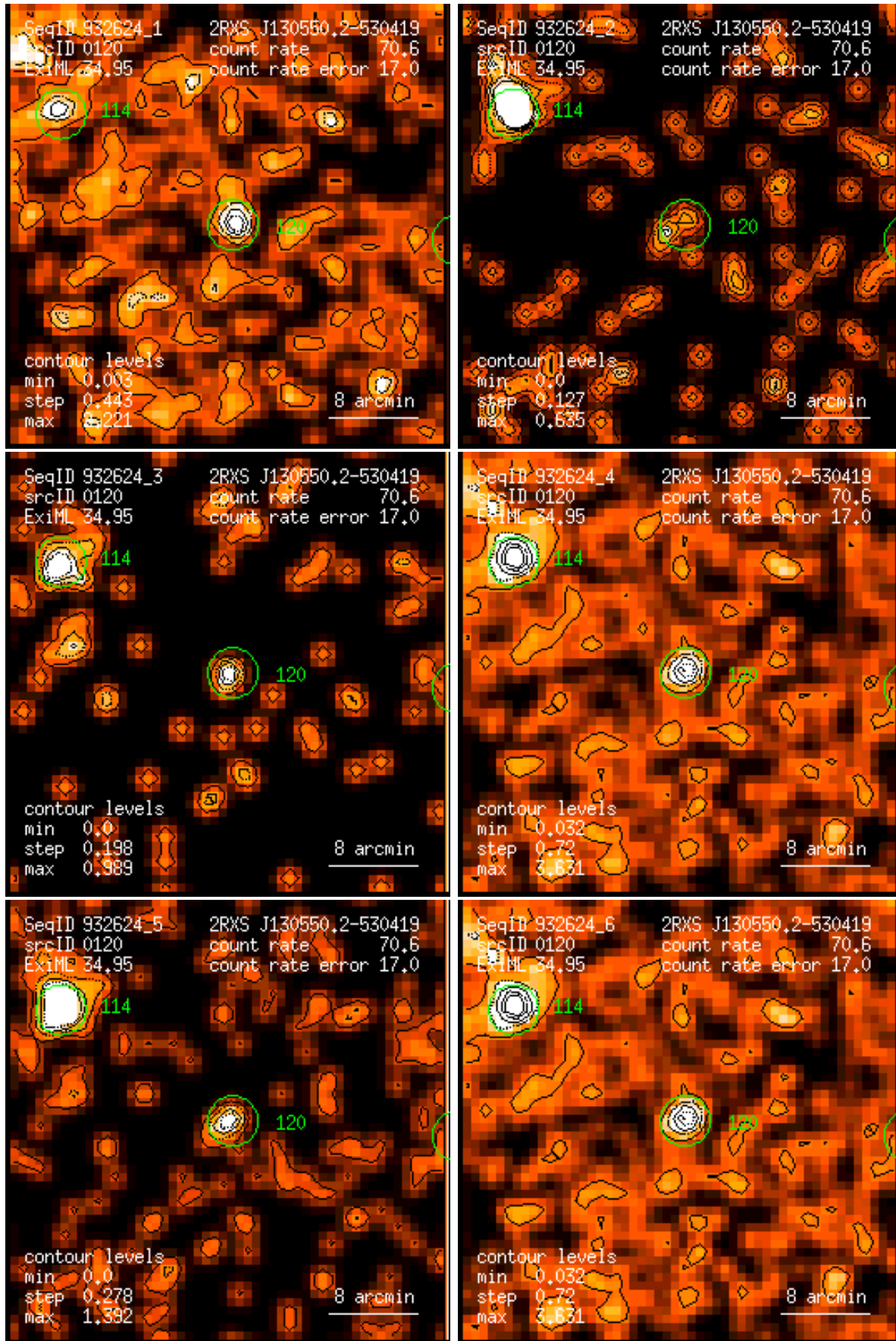
Figure 120: RASS 932624: detection 0120: band rate images, Gaussian filter: (1) PSPC channels 11 – 41, (2) 52 – 90, (3) 91 – 201, (4) 11 – 235, (5) 52 – 201, (6) 11 – 201. Broad band rates in counts/ks. Band rate contour levels in counts/ks/arcmin 2 .
