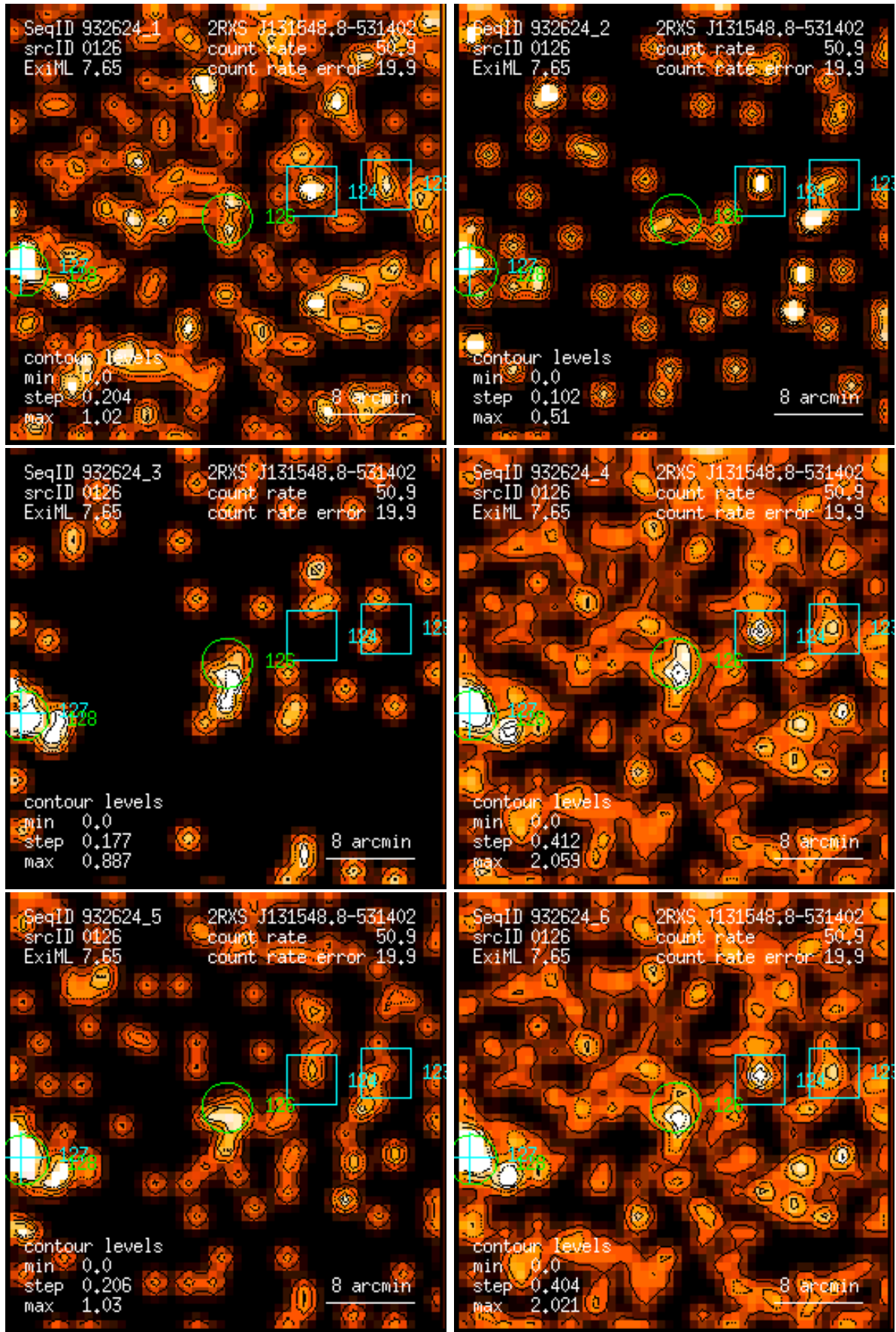
Figure 126: RASS 932624: detection 0126: band rate images, Gaussian filter: (1) PSPC channels 11 – 41, (2) 52 – 90, (3) 91 – 201, (4) 11 – 235, (5) 52 – 201, (6) 11 – 201. Broad band rates in counts/ks. Band rate contour levels in counts/ks/arcmin 2 .
