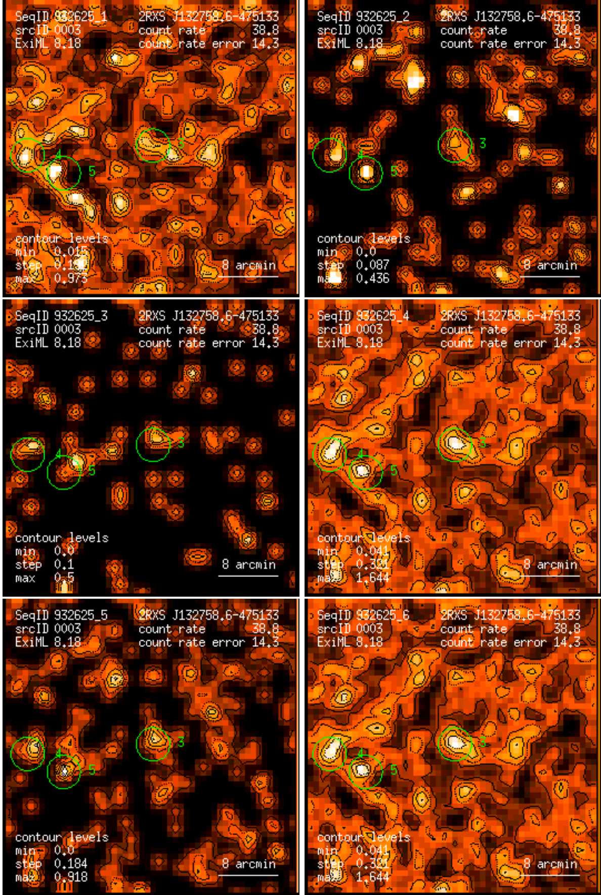
Figure 3: RASS 932625: detection 0003: band rate images, Gaussian filter: (1) PSPC channels 11 – 41, (2) 52 – 90, (3) 91 – 201, (4) 11 – 235, (5) 52 – 201, (6) 11 – 201. Broad band rates in counts/ks. Band rate contour levels in counts/ks/arcmin 2 .
