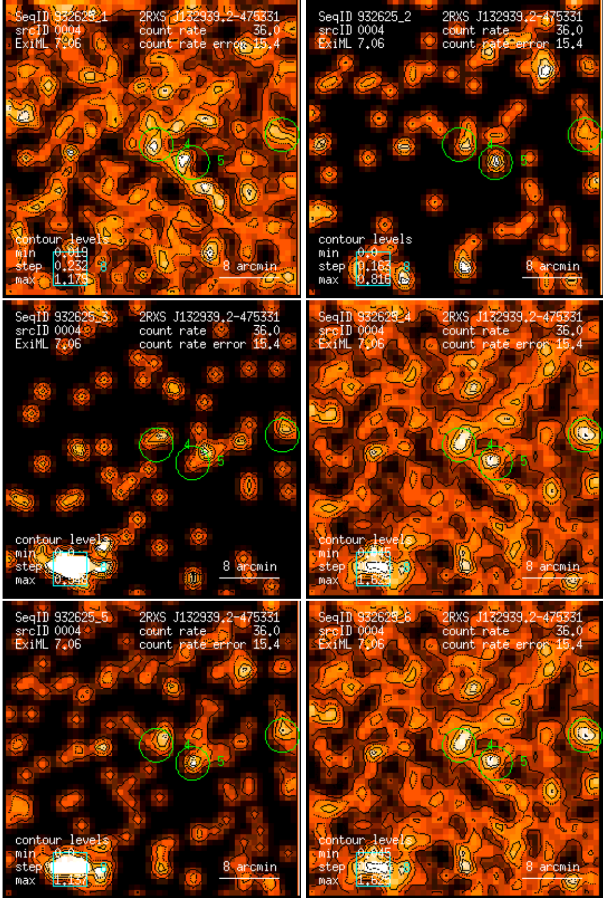
Figure 4: RASS 932625: detection 0004: band rate images, Gaussian filter: (1) PSPC channels 11 – 41, (2) 52 – 90, (3) 91 – 201, (4) 11 – 235, (5) 52 – 201, (6) 11 – 201. Broad band rates in counts/ks. Band rate contour levels in counts/ks/arcmin 2 .
