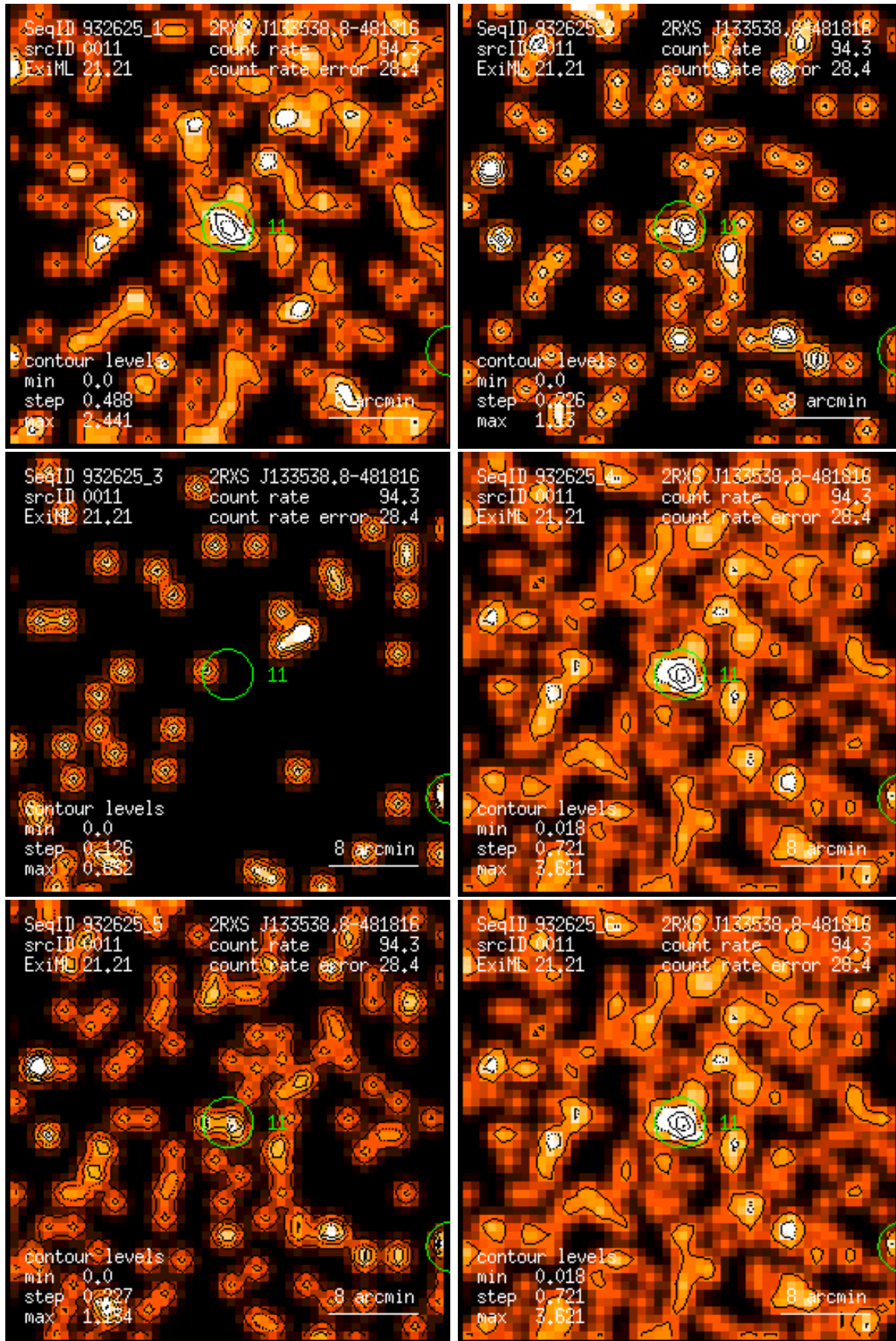
Figure 11: RASS 932625: detection 0011: band rate images, Gaussian filter: (1) PSPC channels 11 – 41, (2) 52 – 90, (3) 91 – 201, (4) 11 – 235, (5) 52 – 201, (6) 11 – 201. Broad band rates in counts/ks. Band rate contour levels in counts/ks/arcmin 2 .
