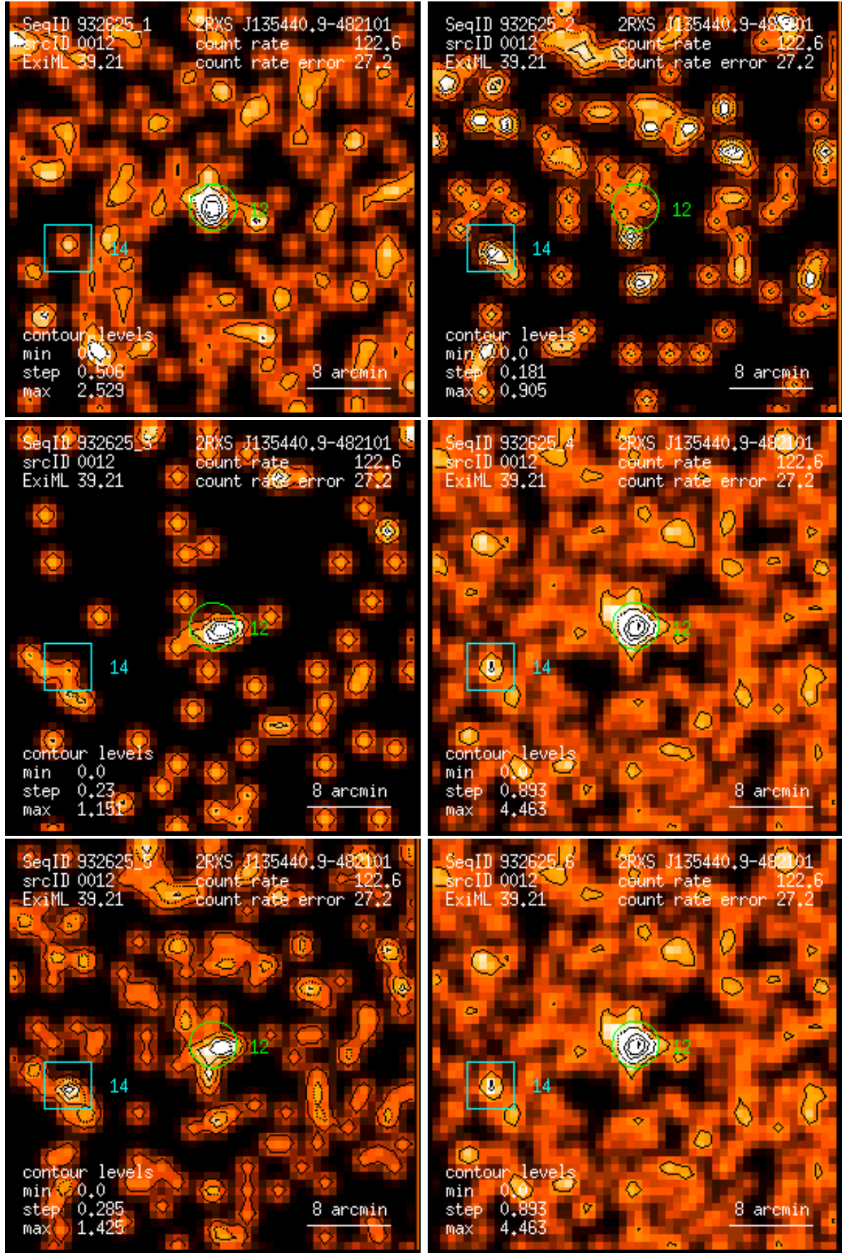
Figure 12: RASS 932625: detection 0012: band rate images, Gaussian filter: (1) PSPC channels 11 – 41, (2) 52 – 90, (3) 91 – 201, (4) 11 – 235, (5) 52 – 201, (6) 11 – 201. Broad band rates in counts/ks. Band rate contour levels in counts/ks/arcmin 2 .
