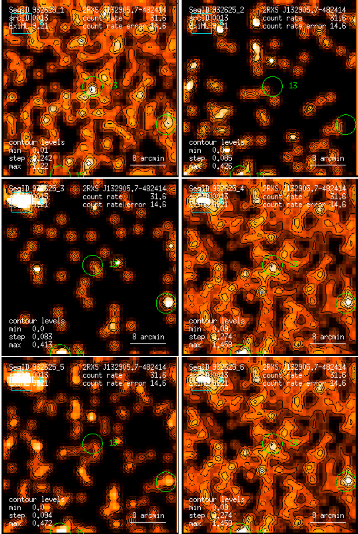
Figure 13: RASS 932625: detection 0013: band rate images, Gaussian filter: (1) PSPC channels 11 – 41, (2) 52 – 90, (3) 91 – 201, (4) 11 – 235, (5) 52 – 201, (6) 11 – 201. Broad band rates in counts/ks. Band rate contour levels in counts/ks/arcmin 2 .
