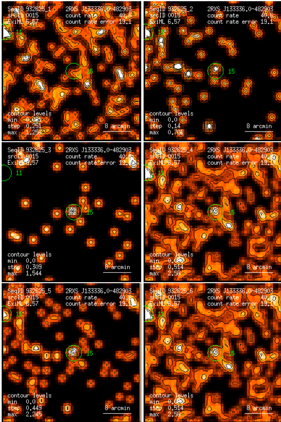
Figure 15: RASS 932625: detection 0015: band rate images, Gaussian filter: (1) PSPC channels 11 – 41, (2) 52 – 90, (3) 91 – 201, (4) 11 – 235, (5) 52 – 201, (6) 11 – 201. Broad band rates in counts/ks. Band rate contour levels in counts/ks/arcmin 2 .
