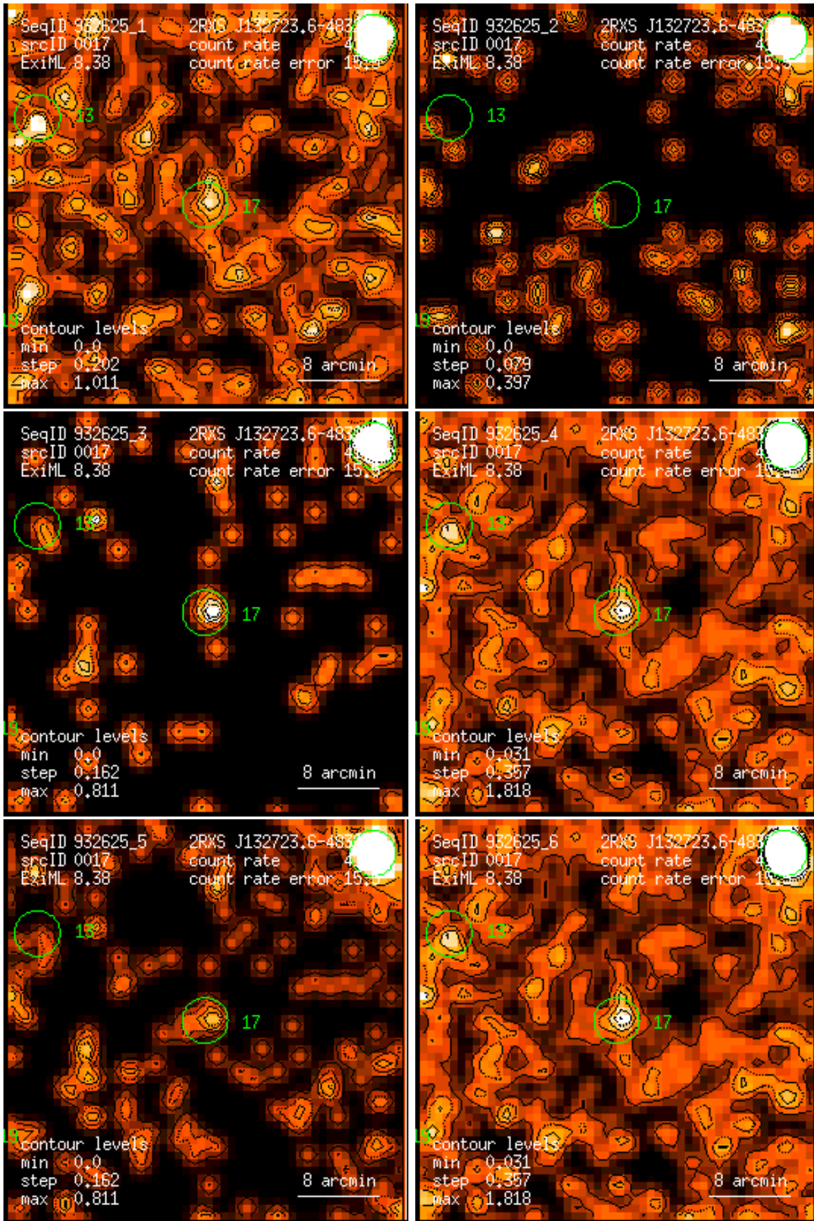
Figure 17: RASS 932625: detection 0017: band rate images, Gaussian filter: (1) PSPC channels 11 – 41, (2) 52 – 90, (3) 91 – 201, (4) 11 – 235, (5) 52 – 201, (6) 11 – 201. Broad band rates in counts/ks. Band rate contour levels in counts/ks/arcmin 2 .
