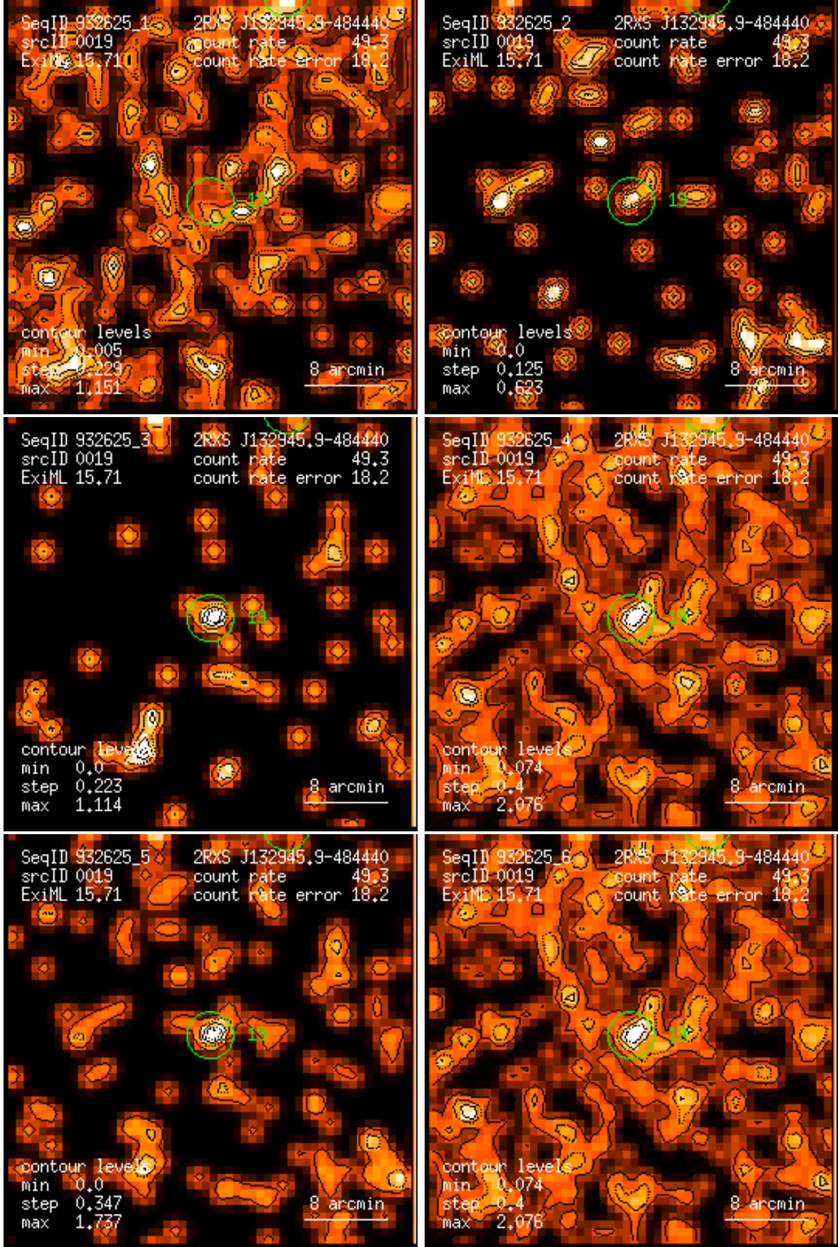
Figure 19: RASS 932625: detection 0019: band rate images, Gaussian filter: (1) PSPC channels 11 – 41, (2) 52 – 90, (3) 91 – 201, (4) 11 – 235, (5) 52 – 201, (6) 11 – 201. Broad band rates in counts/ks. Band rate contour levels in counts/ks/arcmin 2 .
