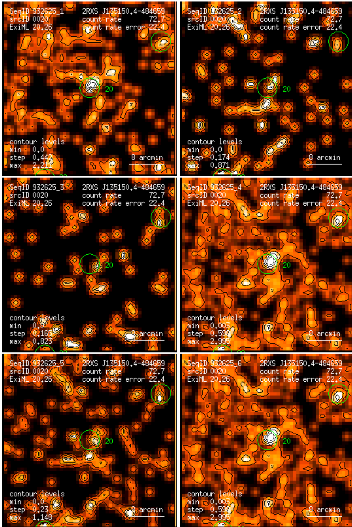
Figure 20: RASS 932625: detection 0020: band rate images, Gaussian filter: (1) PSPC channels 11 – 41, (2) 52 – 90, (3) 91 – 201, (4) 11 – 235, (5) 52 – 201, (6) 11 – 201. Broad band rates in counts/ks. Band rate contour levels in counts/ks/arcmin 2 .
