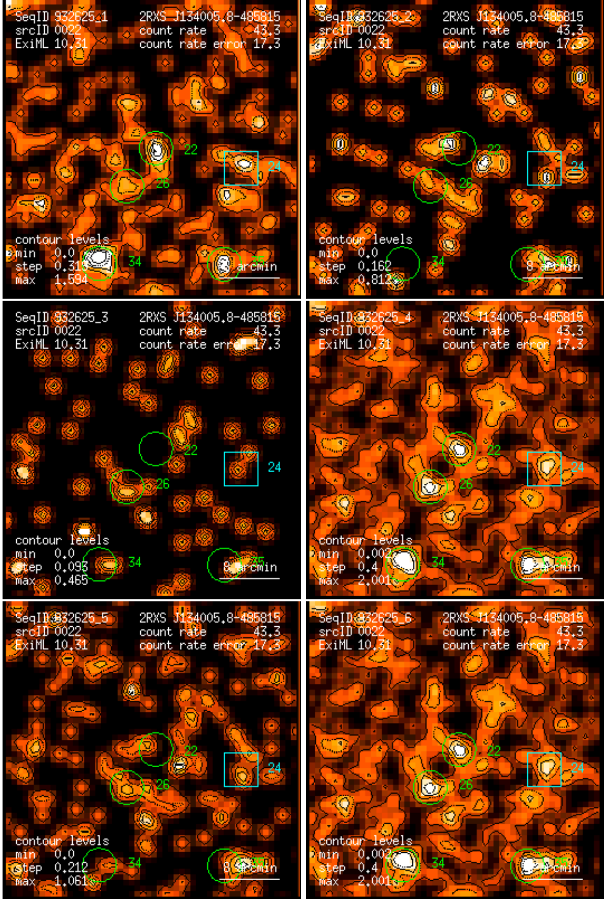
Figure 22: RASS 932625: detection 0022: band rate images, Gaussian filter: (1) PSPC channels 11 – 41, (2) 52 – 90, (3) 91 – 201, (4) 11 – 235, (5) 52 – 201, (6) 11 – 201. Broad band rates in counts/ks. Band rate contour levels in counts/ks/arcmin 2 .
