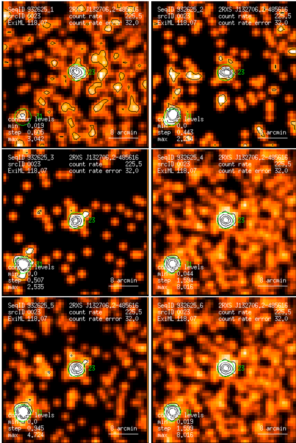
Figure 23: RASS 932625: detection 0023: band rate images, Gaussian filter: (1) PSPC channels 11 – 41, (2) 52 – 90, (3) 91 – 201, (4) 11 – 235, (5) 52 – 201, (6) 11 – 201. Broad band rates in counts/ks. Band rate contour levels in counts/ks/arcmin 2 .
