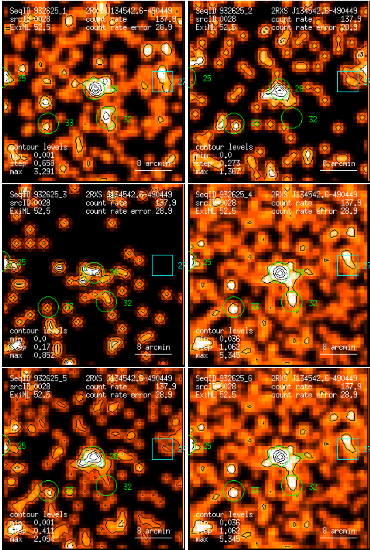
Figure 28: RASS 932625: detection 0028: band rate images, Gaussian filter: (1) PSPC channels 11 – 41, (2) 52 – 90, (3) 91 – 201, (4) 11 – 235, (5) 52 – 201, (6) 11 – 201. Broad band rates in counts/ks. Band rate contour levels in counts/ks/arcmin 2 .
