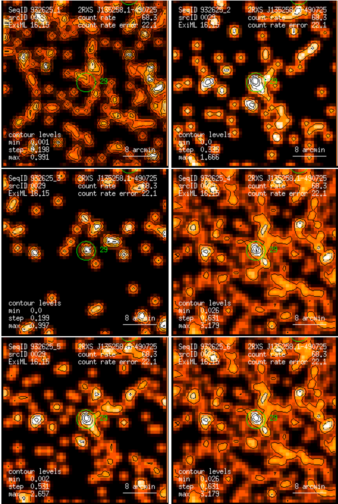
Figure 29: RASS 932625: detection 0029: band rate images, Gaussian filter: (1) PSPC channels 11 – 41, (2) 52 – 90, (3) 91 – 201, (4) 11 – 235, (5) 52 – 201, (6) 11 – 201. Broad band rates in counts/ks. Band rate contour levels in counts/ks/arcmin 2 .
