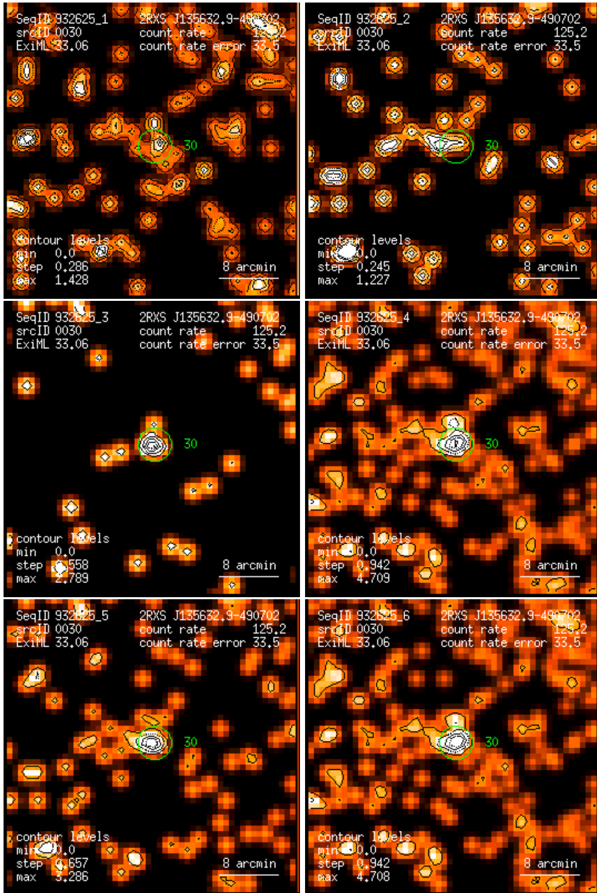
Figure 30: RASS 932625: detection 0030: band rate images, Gaussian filter: (1) PSPC channels 11 – 41, (2) 52 – 90, (3) 91 – 201, (4) 11 – 235, (5) 52 – 201, (6) 11 – 201. Broad band rates in counts/ks. Band rate contour levels in counts/ks/arcmin 2 .
