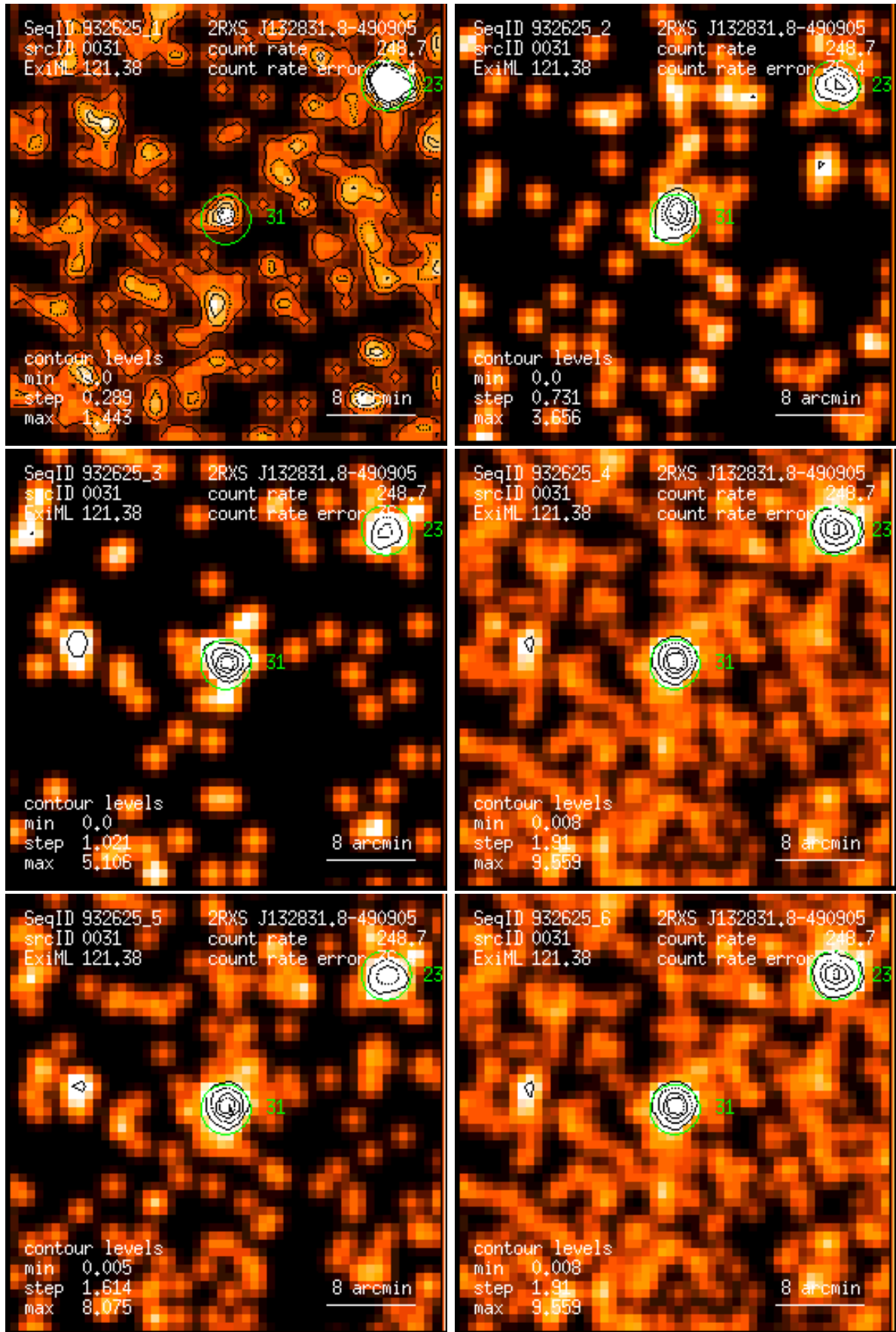
Figure 31: RASS 932625: detection 0031: band rate images, Gaussian filter: (1) PSPC channels 11 – 41, (2) 52 – 90, (3) 91 – 201, (4) 11 – 235, (5) 52 – 201, (6) 11 – 201. Broad band rates in counts/ks. Band rate contour levels in counts/ks/arcmin 2 .
