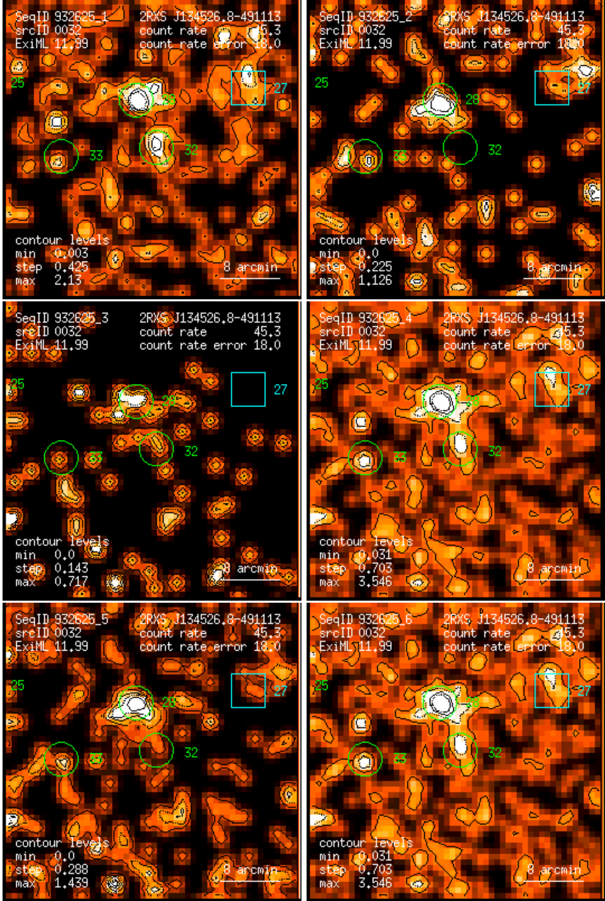
Figure 32: RASS 932625: detection 0032: band rate images, Gaussian filter: (1) PSPC channels 11 – 41, (2) 52 – 90, (3) 91 – 201, (4) 11 – 235, (5) 52 – 201, (6) 11 – 201. Broad band rates in counts/ks. Band rate contour levels in counts/ks/arcmin 2 .
