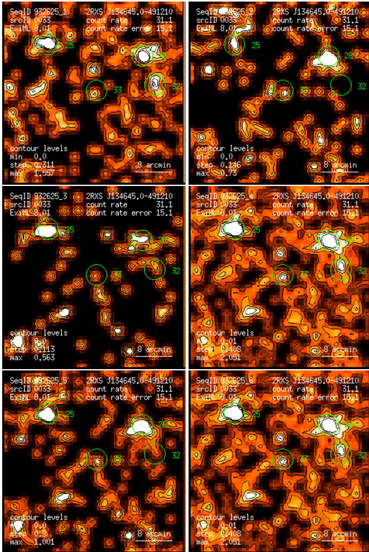
Figure 33: RASS 932625: detection 0033: band rate images, Gaussian filter: (1) PSPC channels 11 – 41, (2) 52 – 90, (3) 91 – 201, (4) 11 – 235, (5) 52 – 201, (6) 11 – 201. Broad band rates in counts/ks. Band rate contour levels in counts/ks/arcmin 2 .
