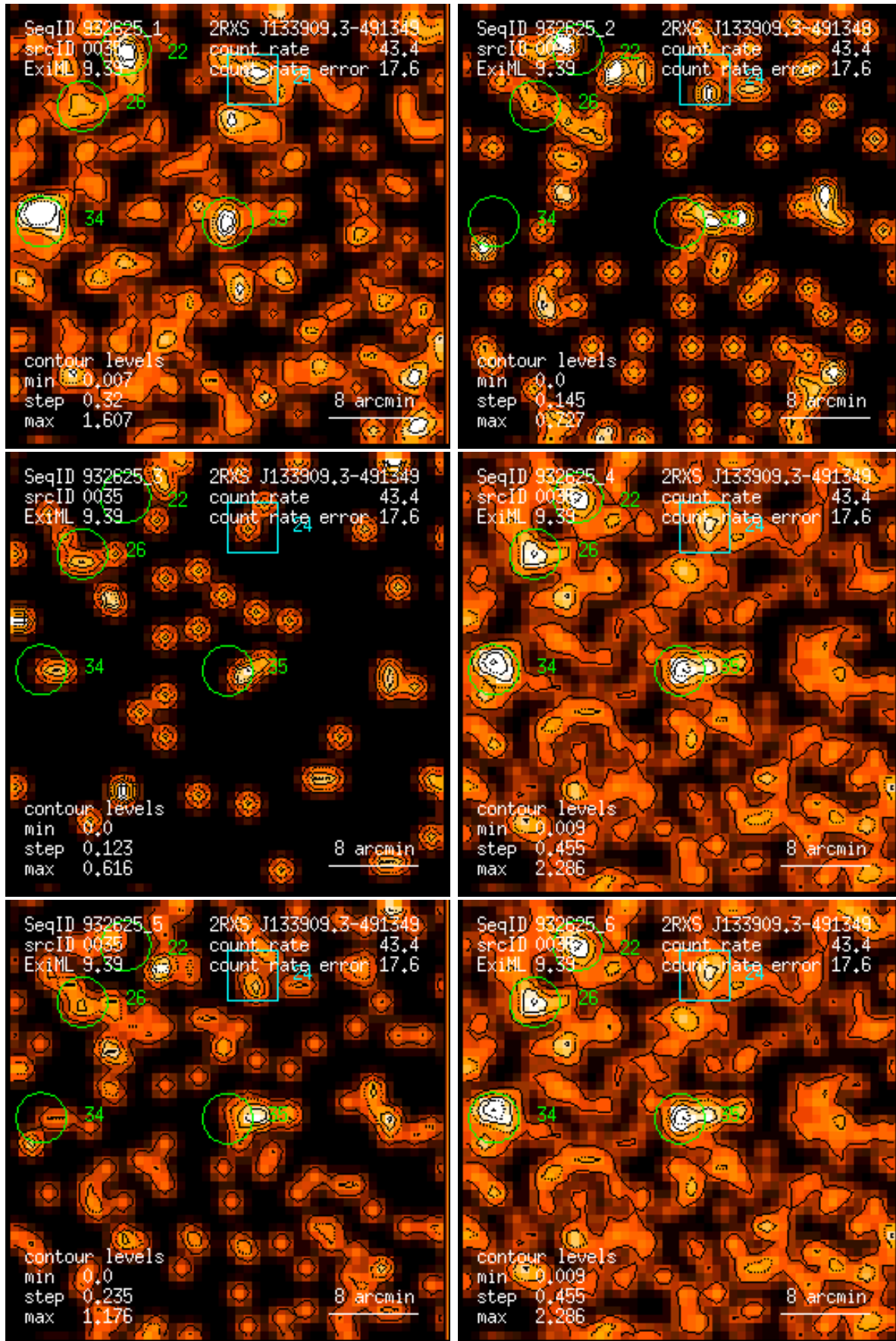
Figure 35: RASS 932625: detection 0035: band rate images, Gaussian filter: (1) PSPC channels 11 – 41, (2) 52 – 90, (3) 91 – 201, (4) 11 – 235, (5) 52 – 201, (6) 11 – 201. Broad band rates in counts/ks. Band rate contour levels in counts/ks/arcmin 2 .
