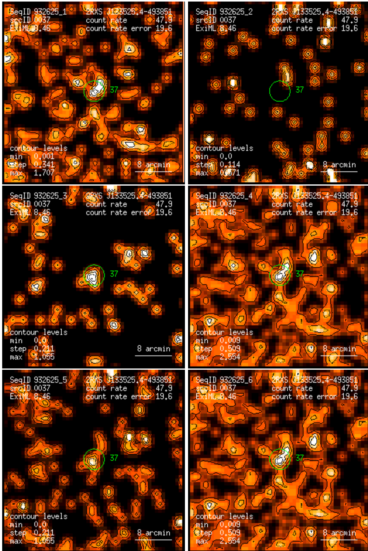
Figure 37: RASS 932625: detection 0037: band rate images, Gaussian filter: (1) PSPC channels 11 – 41, (2) 52 – 90, (3) 91 – 201, (4) 11 – 235, (5) 52 – 201, (6) 11 – 201. Broad band rates in counts/ks. Band rate contour levels in counts/ks/arcmin 2 .
