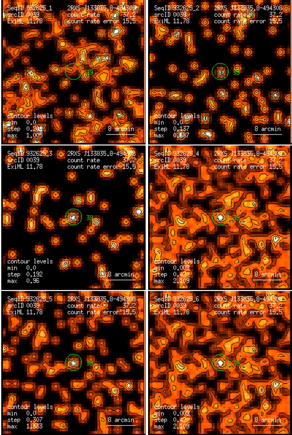
Figure 39: RASS 932625: detection 0039: band rate images, Gaussian filter: (1) PSPC channels 11 – 41, (2) 52 – 90, (3) 91 – 201, (4) 11 – 235, (5) 52 – 201, (6) 11 – 201. Broad band rates in counts/ks. Band rate contour levels in counts/ks/arcmin 2 .
