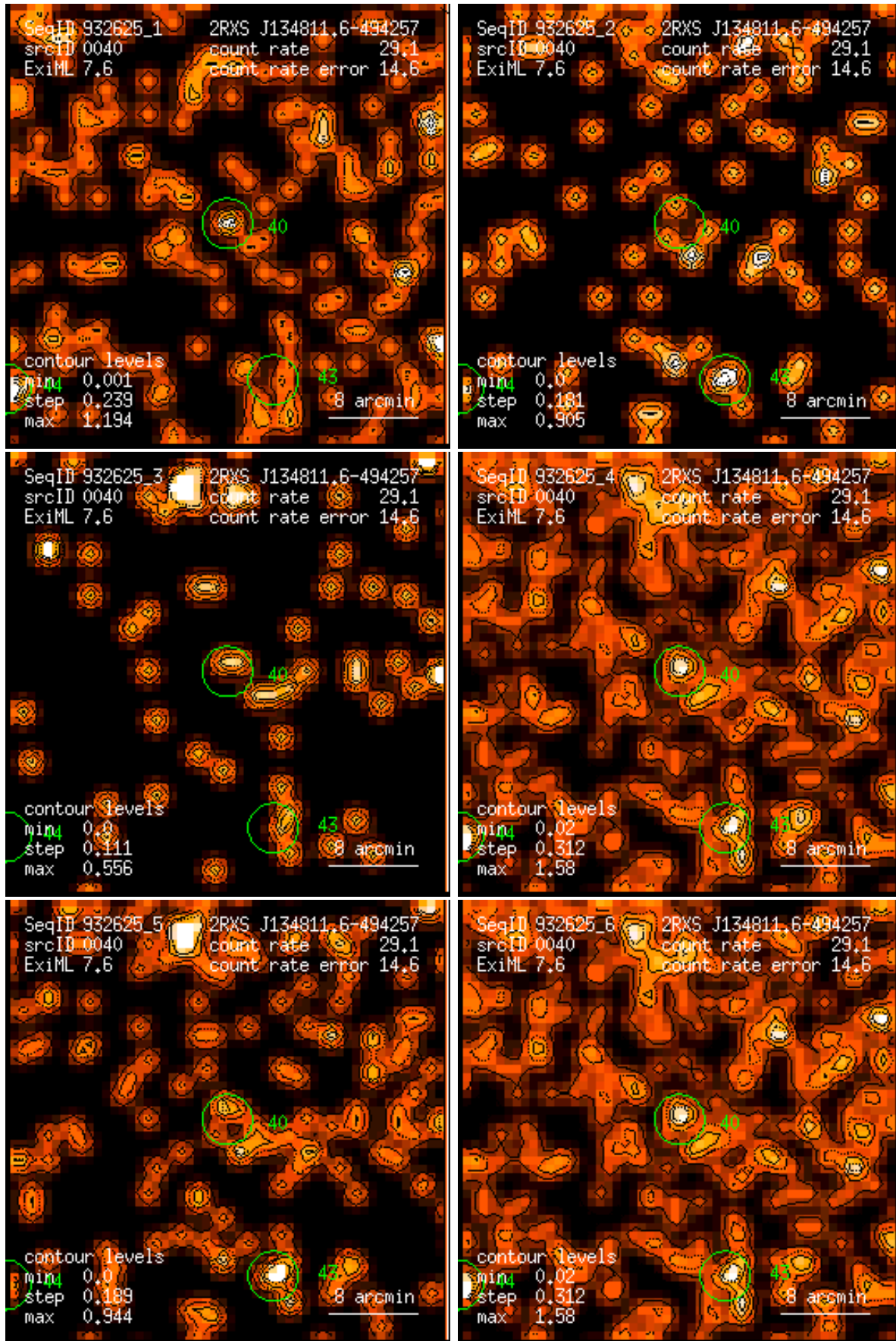
Figure 40: RASS 932625: detection 0040: band rate images, Gaussian filter: (1) PSPC channels 11 – 41, (2) 52 – 90, (3) 91 – 201, (4) 11 – 235, (5) 52 – 201, (6) 11 – 201. Broad band rates in counts/ks. Band rate contour levels in counts/ks/arcmin 2 .
