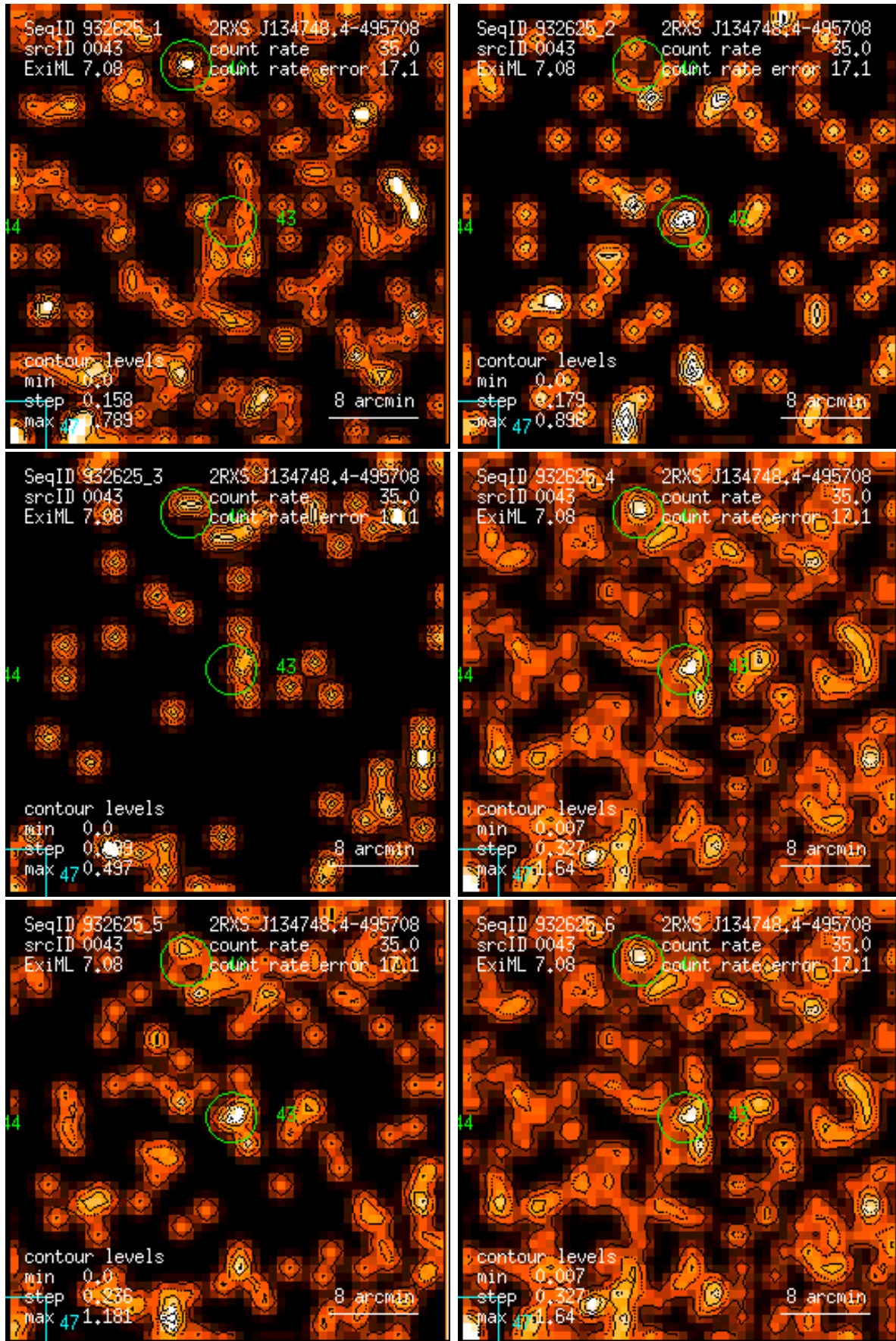
Figure 43: RASS 932625: detection 0043: band rate images, Gaussian filter: (1) PSPC channels 11 – 41, (2) 52 – 90, (3) 91 – 201, (4) 11 – 235, (5) 52 – 201, (6) 11 – 201. Broad band rates in counts/ks. Band rate contour levels in counts/ks/arcmin 2 .
