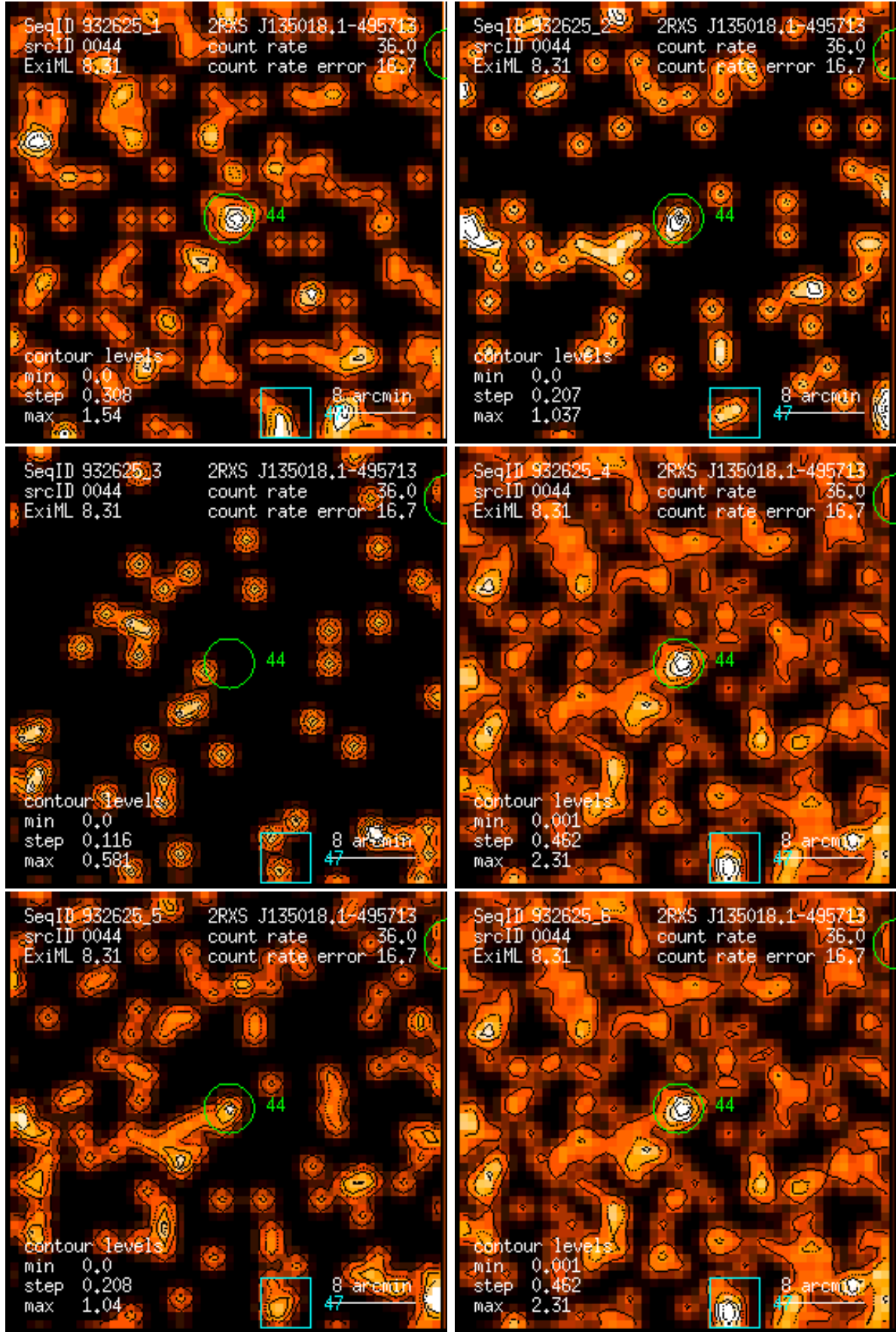
Figure 44: RASS 932625: detection 0044: band rate images, Gaussian filter: (1) PSPC channels 11 – 41, (2) 52 – 90, (3) 91 – 201, (4) 11 – 235, (5) 52 – 201, (6) 11 – 201. Broad band rates in counts/ks. Band rate contour levels in counts/ks/arcmin 2 .
