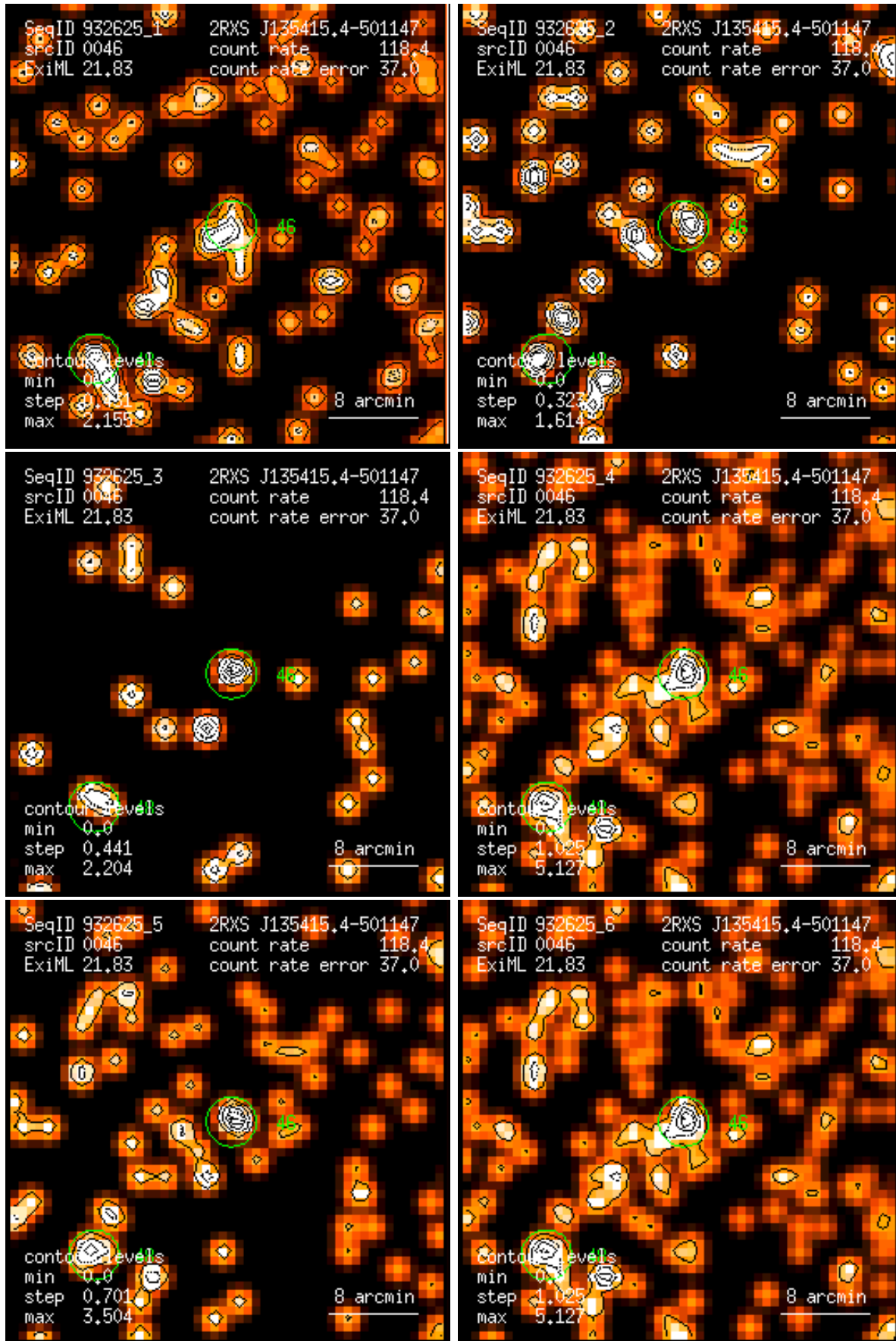
Figure 46: RASS 932625: detection 0046: band rate images, Gaussian filter: (1) PSPC channels 11 – 41, (2) 52 – 90, (3) 91 – 201, (4) 11 – 235, (5) 52 – 201, (6) 11 – 201. Broad band rates in counts/ks. Band rate contour levels in counts/ks/arcmin 2 .
