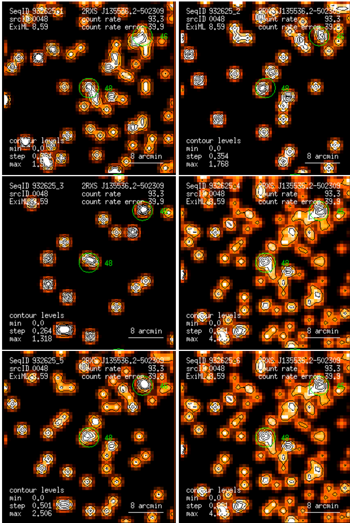
Figure 48: RASS 932625: detection 0048: band rate images, Gaussian filter: (1) PSPC channels 11 – 41, (2) 52 – 90, (3) 91 – 201, (4) 11 – 235, (5) 52 – 201, (6) 11 – 201. Broad band rates in counts/ks. Band rate contour levels in counts/ks/arcmin 2 .
