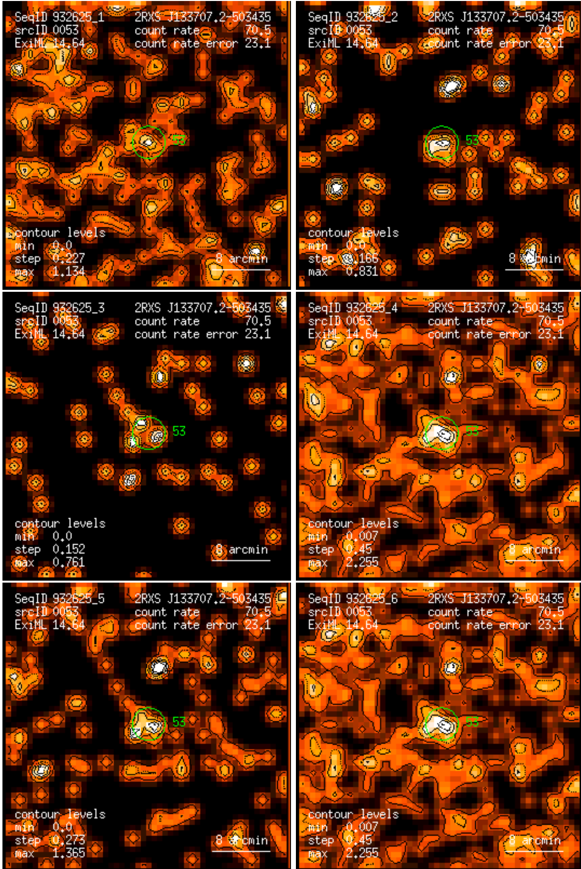
Figure 53: RASS 932625: detection 0053: band rate images, Gaussian filter: (1) PSPC channels 11 – 41, (2) 52 – 90, (3) 91 – 201, (4) 11 – 235, (5) 52 – 201, (6) 11 – 201. Broad band rates in counts/ks. Band rate contour levels in counts/ks/arcmin 2 .
