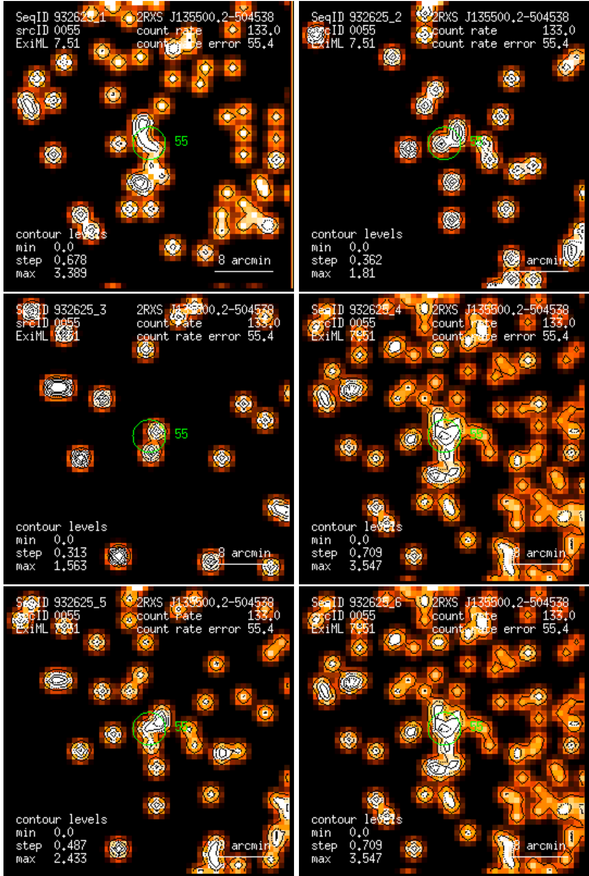
Figure 55: RASS 932625: detection 0055: band rate images, Gaussian filter: (1) PSPC channels 11 – 41, (2) 52 – 90, (3) 91 – 201, (4) 11 – 235, (5) 52 – 201, (6) 11 – 201. Broad band rates in counts/ks. Band rate contour levels in counts/ks/arcmin 2 .
