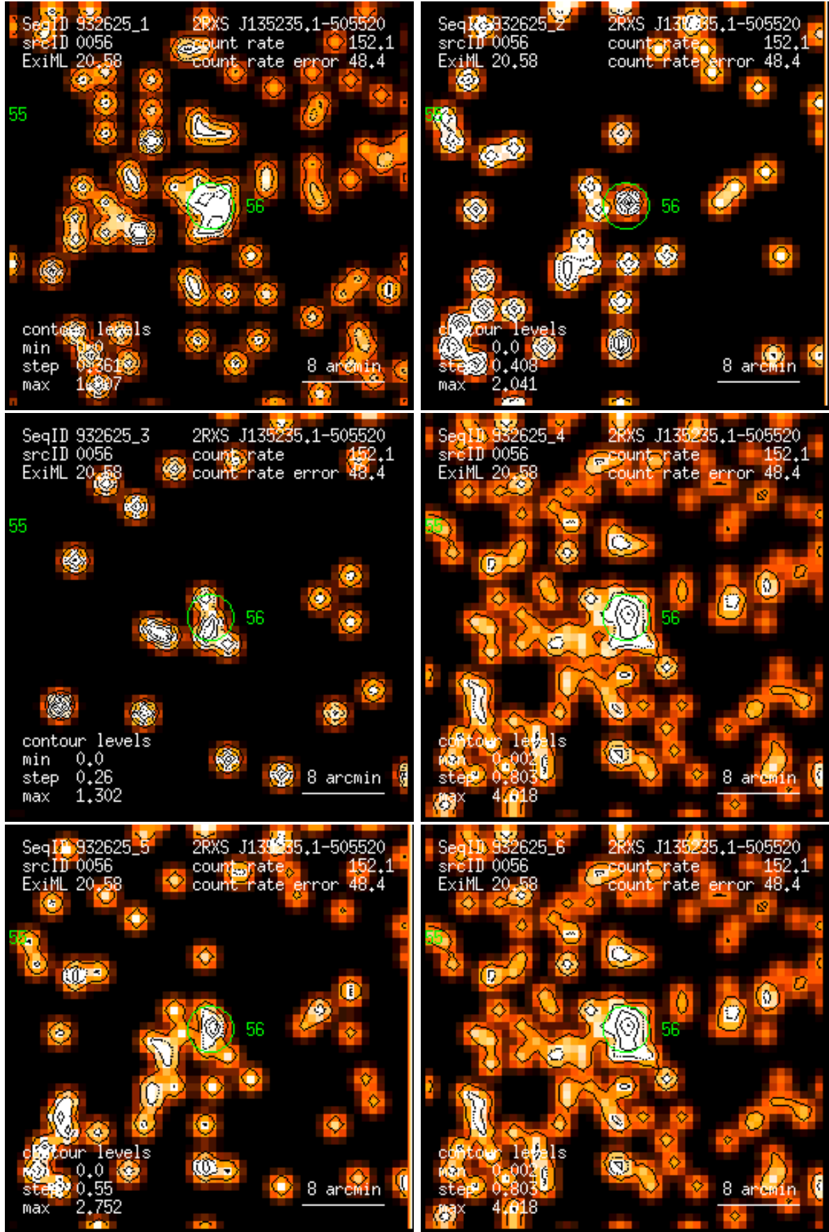
Figure 56: RASS 932625: detection 0056: band rate images, Gaussian filter: (1) PSPC channels 11 – 41, (2) 52 – 90, (3) 91 – 201, (4) 11 – 235, (5) 52 – 201, (6) 11 – 201. Broad band rates in counts/ks. Band rate contour levels in counts/ks/arcmin 2 .
