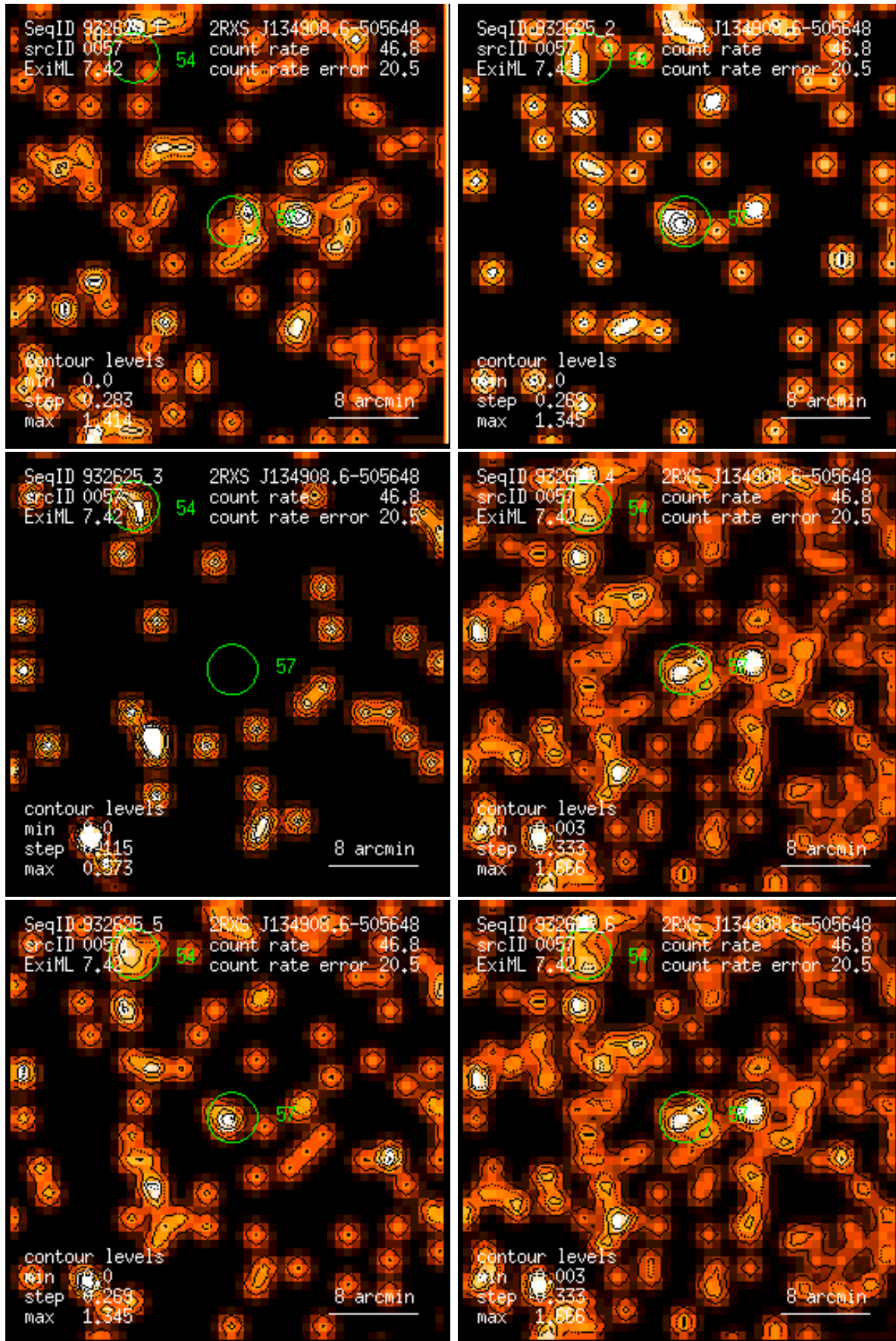
Figure 57: RASS 932625: detection 0057: band rate images, Gaussian filter: (1) PSPC channels 11 – 41, (2) 52 – 90, (3) 91 – 201, (4) 11 – 235, (5) 52 – 201, (6) 11 – 201. Broad band rates in counts/ks. Band rate contour levels in counts/ks/arcmin 2 .
