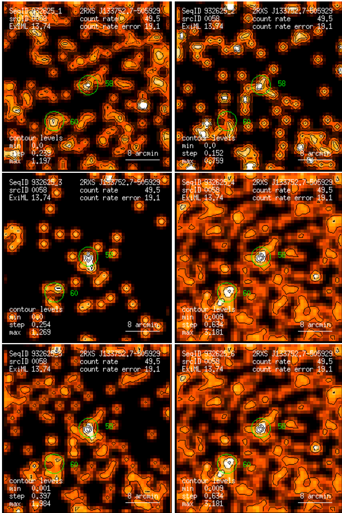
Figure 58: RASS 932625: detection 0058: band rate images, Gaussian filter: (1) PSPC channels 11 – 41, (2) 52 – 90, (3) 91 – 201, (4) 11 – 235, (5) 52 – 201, (6) 11 – 201. Broad band rates in counts/ks. Band rate contour levels in counts/ks/arcmin 2 .
