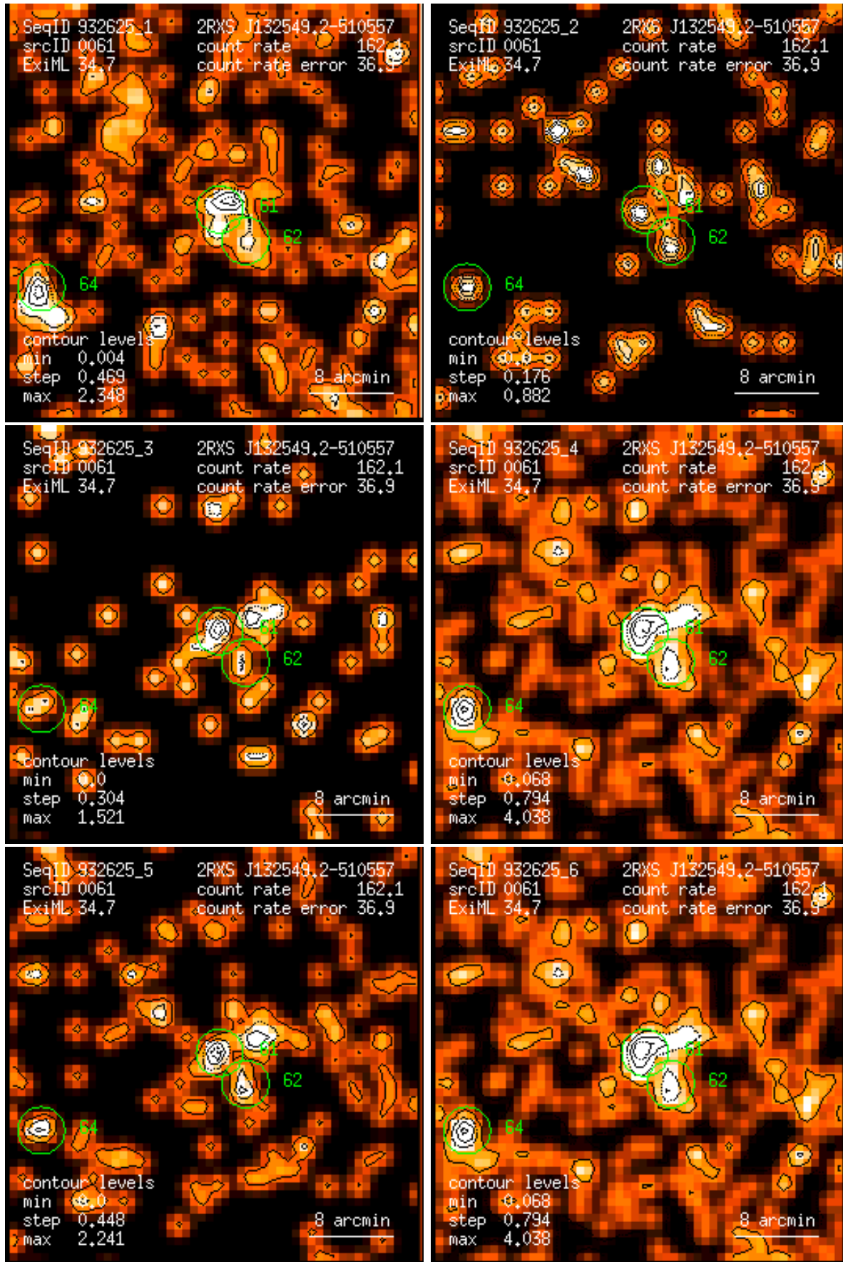
Figure 61: RASS 932625: detection 0061: band rate images, Gaussian filter: (1) PSPC channels 11 – 41, (2) 52 – 90, (3) 91 – 201, (4) 11 – 235, (5) 52 – 201, (6) 11 – 201. Broad band rates in counts/ks. Band rate contour levels in counts/ks/arcmin 2 .
