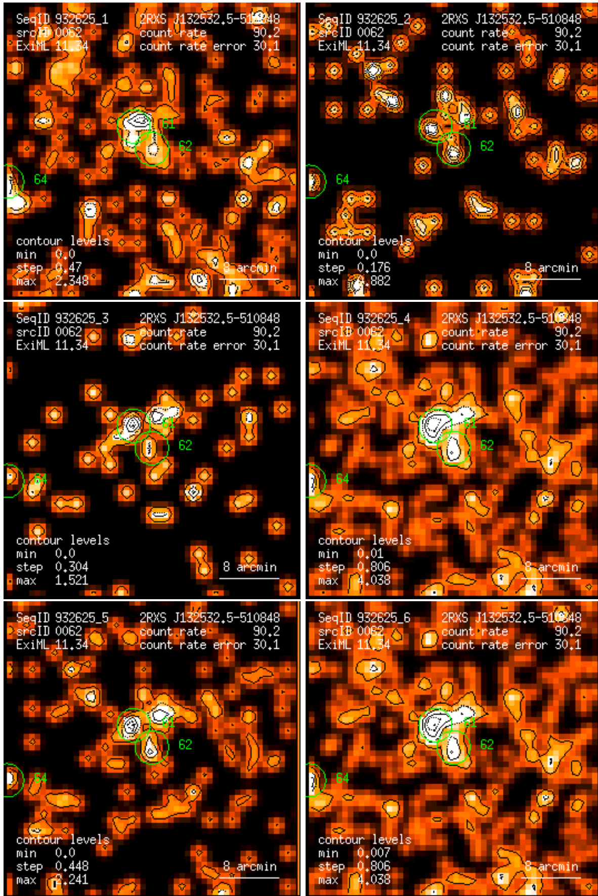
Figure 62: RASS 932625: detection 0062: band rate images, Gaussian filter: (1) PSPC channels 11 – 41, (2) 52 – 90, (3) 91 – 201, (4) 11 – 235, (5) 52 – 201, (6) 11 – 201. Broad band rates in counts/ks. Band rate contour levels in counts/ks/arcmin 2 .
