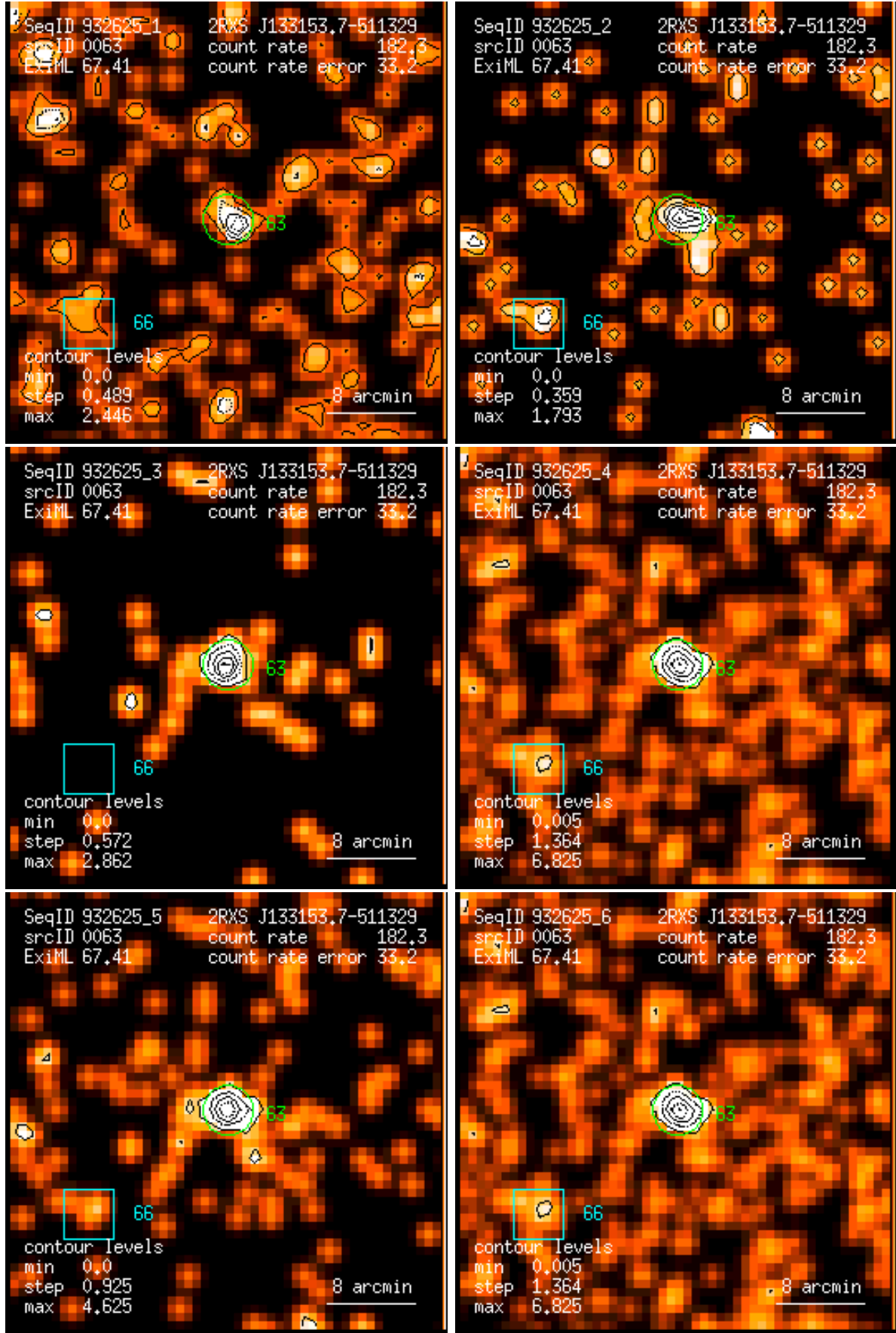
Figure 63: RASS 932625: detection 0063: band rate images, Gaussian filter: (1) PSPC channels 11 – 41, (2) 52 – 90, (3) 91 – 201, (4) 11 – 235, (5) 52 – 201, (6) 11 – 201. Broad band rates in counts/ks. Band rate contour levels in counts/ks/arcmin 2 .
