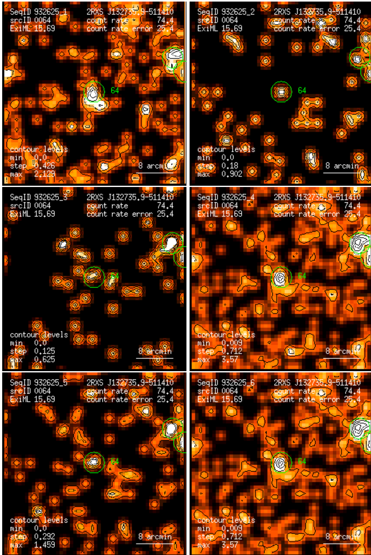
Figure 64: RASS 932625: detection 0064: band rate images, Gaussian filter: (1) PSPC channels 11 – 41, (2) 52 – 90, (3) 91 – 201, (4) 11 – 235, (5) 52 – 201, (6) 11 – 201. Broad band rates in counts/ks. Band rate contour levels in counts/ks/arcmin 2 .
