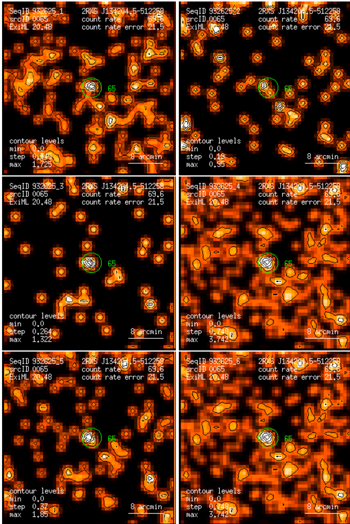
Figure 65: RASS 932625: detection 0065: band rate images, Gaussian filter: (1) PSPC channels 11 – 41, (2) 52 – 90, (3) 91 – 201, (4) 11 – 235, (5) 52 – 201, (6) 11 – 201. Broad band rates in counts/ks. Band rate contour levels in counts/ks/arcmin 2 .
