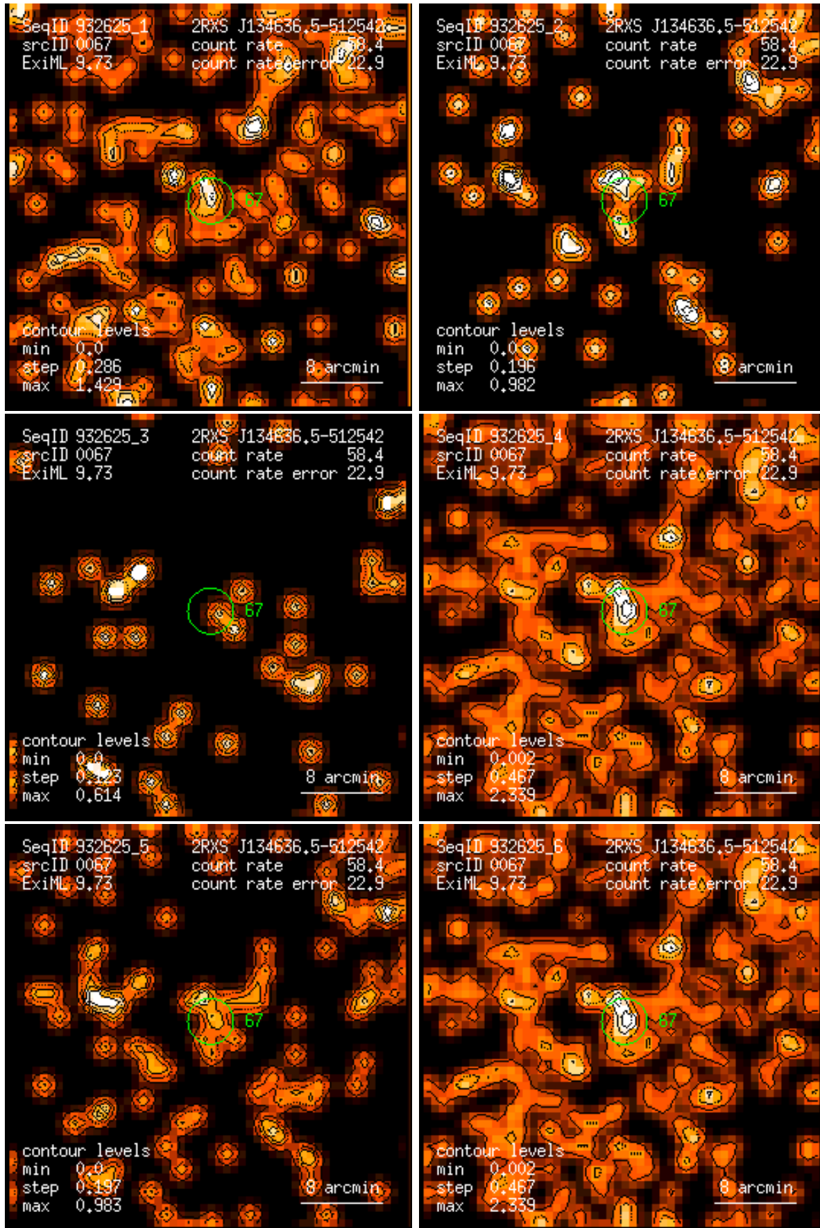
Figure 67: RASS 932625: detection 0067: band rate images, Gaussian filter: (1) PSPC channels 11 – 41, (2) 52 – 90, (3) 91 – 201, (4) 11 – 235, (5) 52 – 201, (6) 11 – 201. Broad band rates in counts/ks. Band rate contour levels in counts/ks/arcmin 2 .
