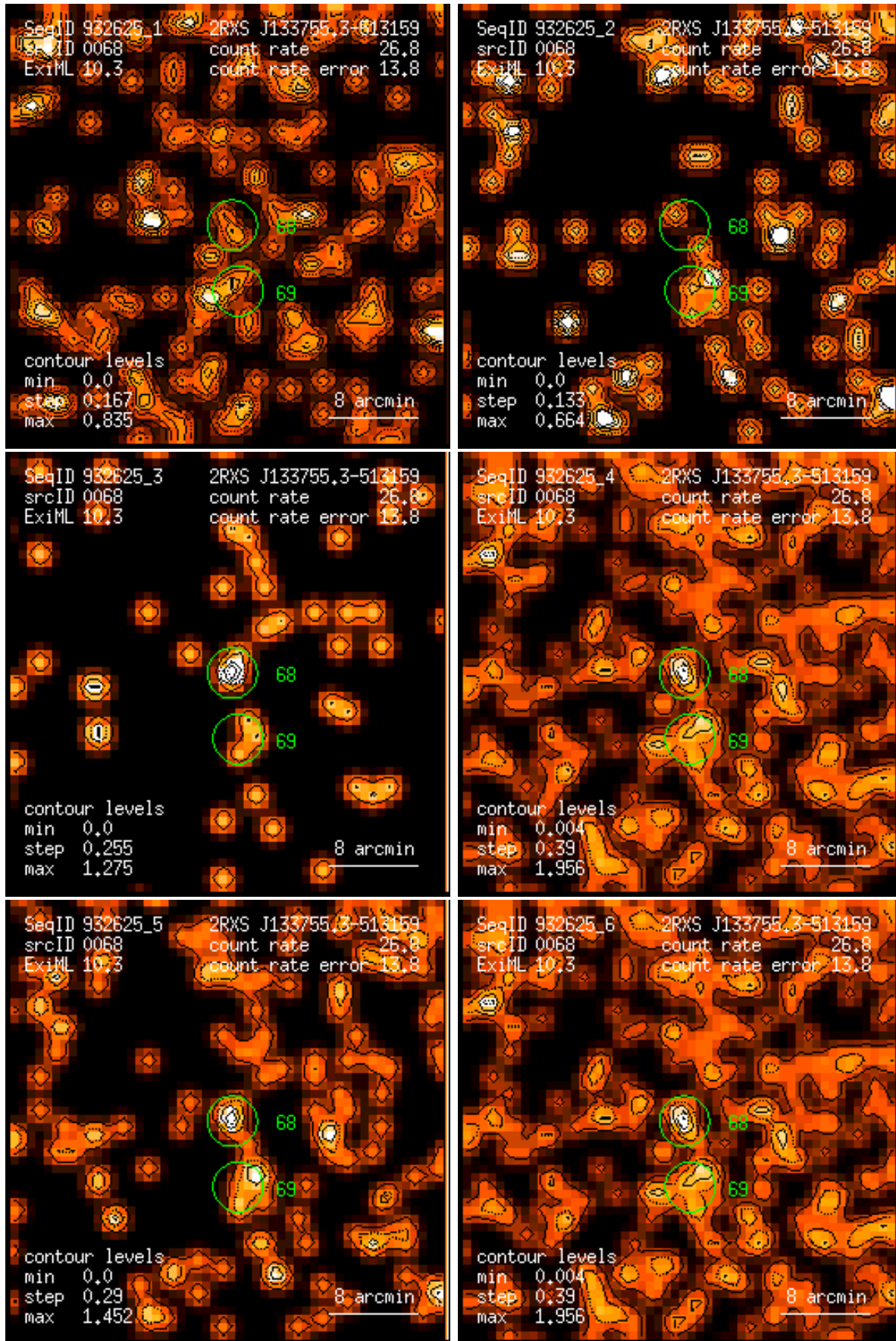
Figure 68: RASS 932625: detection 0068: band rate images, Gaussian filter: (1) PSPC channels 11 – 41, (2) 52 – 90, (3) 91 – 201, (4) 11 – 235, (5) 52 – 201, (6) 11 – 201. Broad band rates in counts/ks. Band rate contour levels in counts/ks/arcmin 2 .
